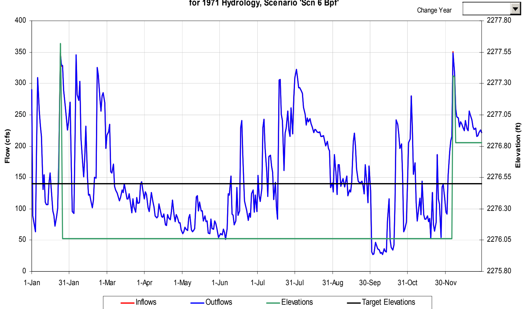
Tuckasegee Reservoir Operational Details for 1971 Hydrology, Scenario 'Scn 6 Bpf'
