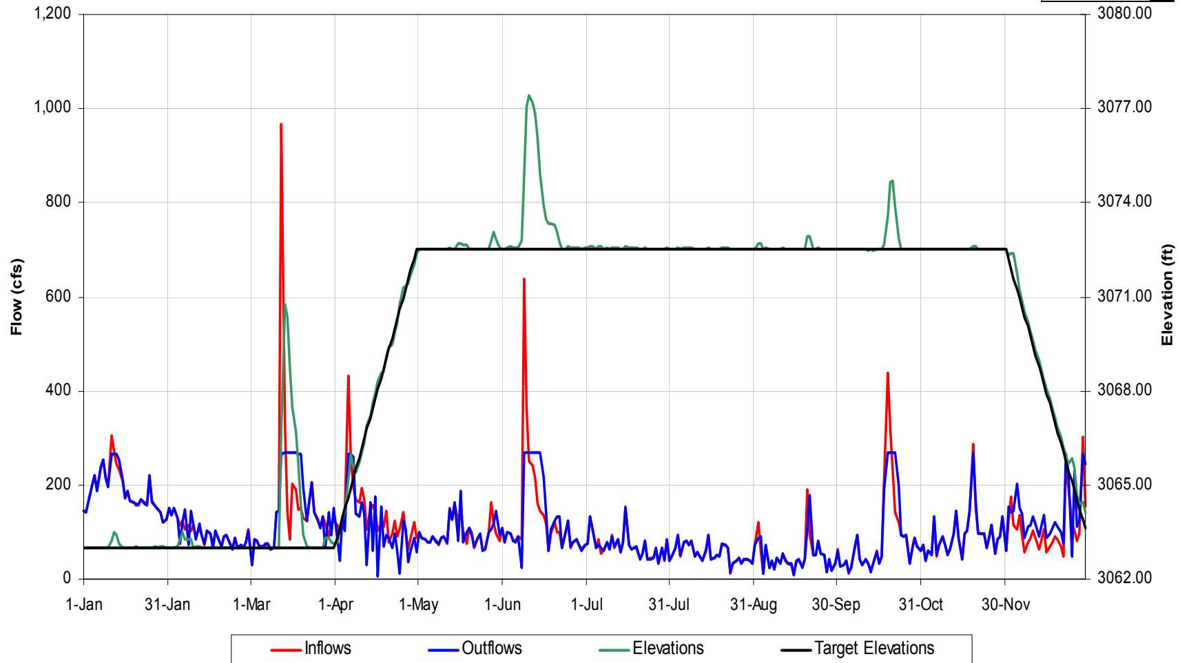
Tennessee Creek Reservoir Operational Details for 1968 Hydrology, Scenario 'Scn 5 Rec Flows_'
