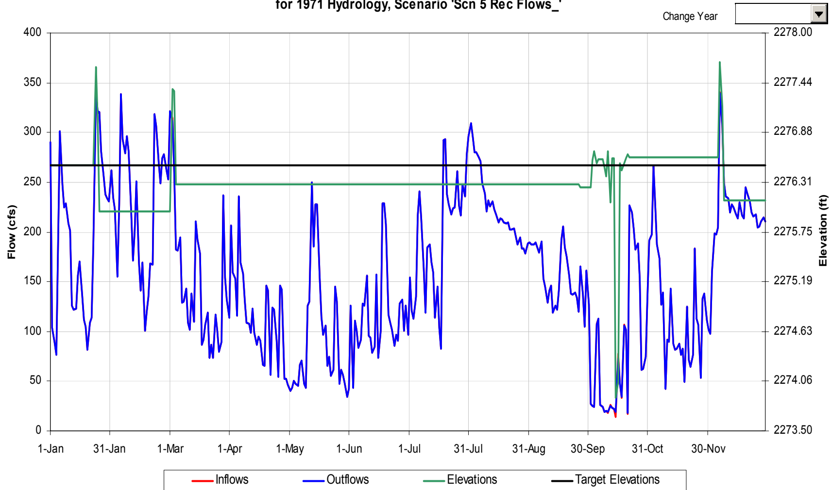
Tuckasegee Reservoir Operational Details for 1971 Hydrology, Scenario 'Scn 5 Rec Flows_'
