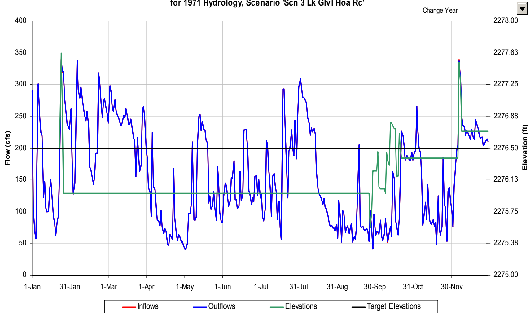
Tuckasegee Reservoir Operational Details for 1971 Hydrology, Scenario 'Scn 3 Lk Glvl Hoa Rc'
