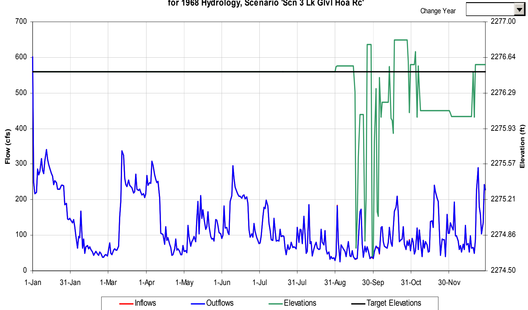
Tuckasegee Reservoir Operational Details for 1968 Hydrology, Scenario 'Scn 3 Lk Glvl Hoa Rc'
