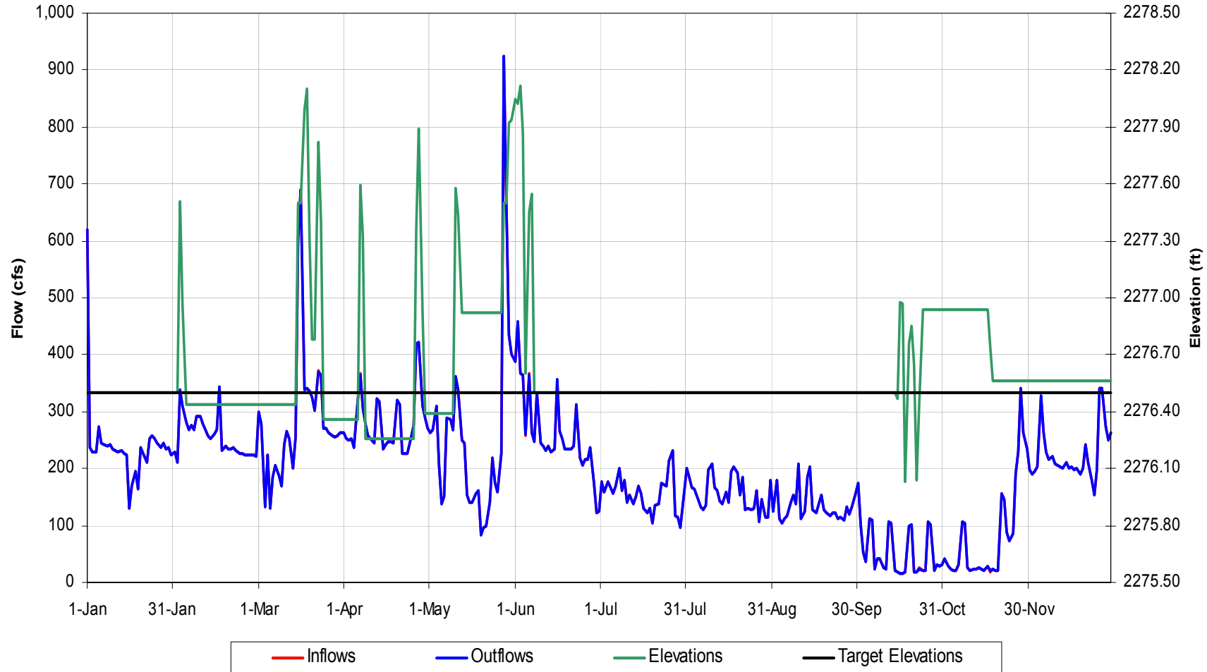
Tuckasegee Reservoir Operational Details for 1973 Hydrology, Scenario 'Scn 5a 2xrec Flows'
