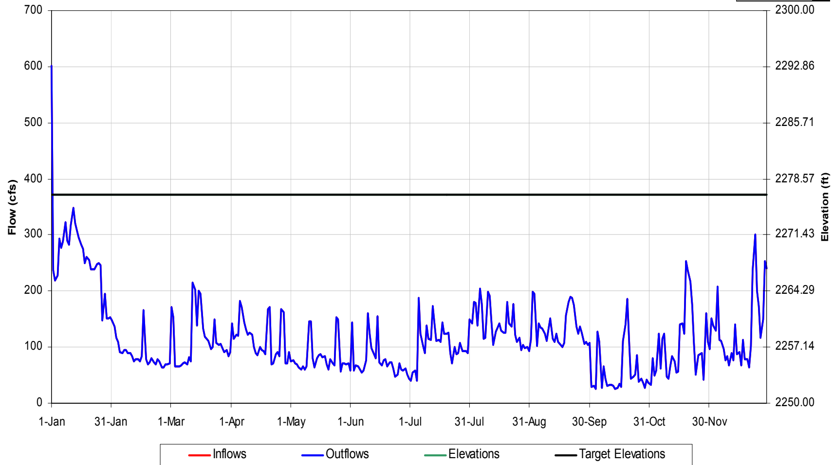
Tuckasegee Reservoir Operational Details for 1968 Hydrology, Scenario 'Scn7 Bpf_'
