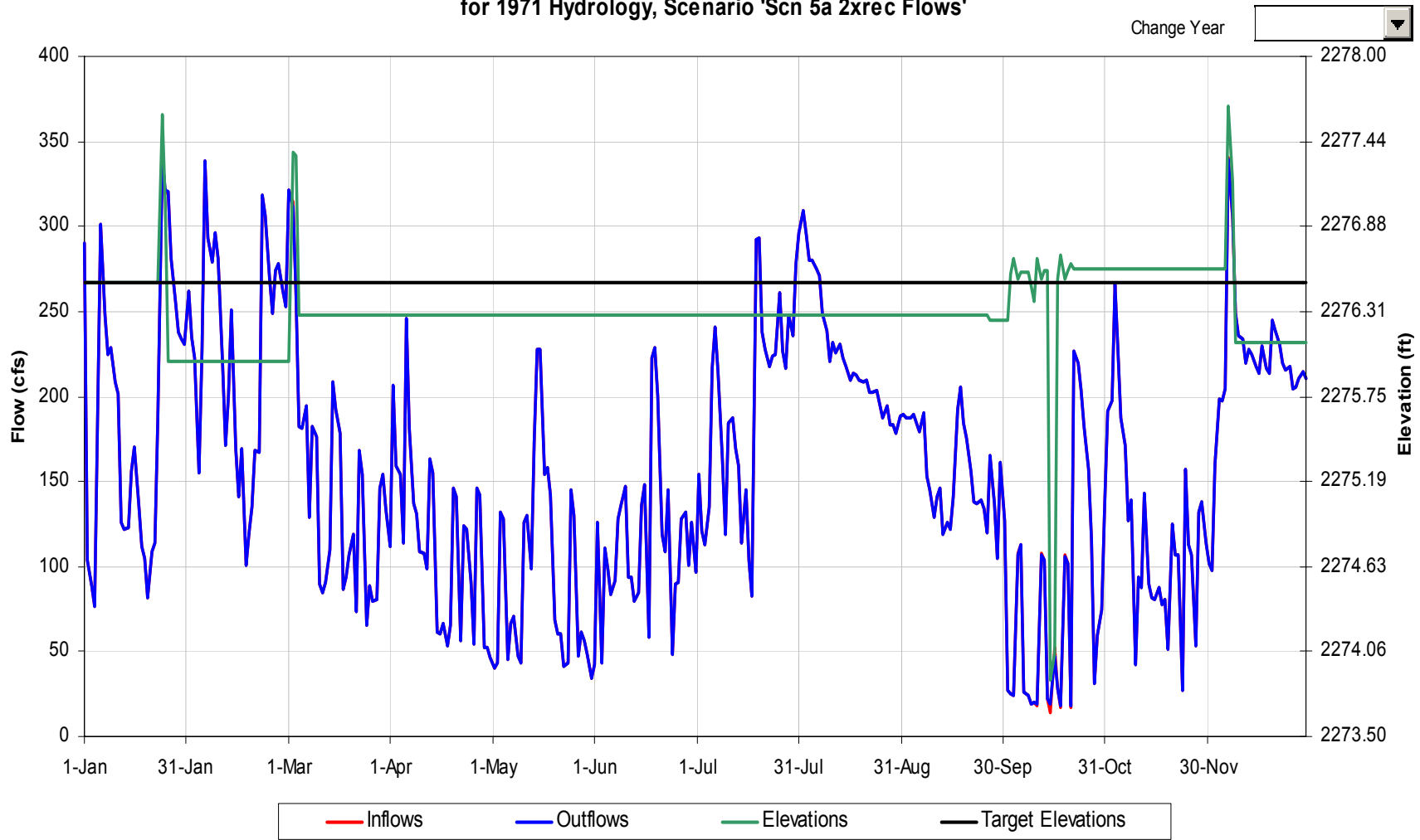
Tuckasegee Reservoir Operational Details for 1971 Hydrology, Scenario 'Scn 5a 2xrec Flows'
