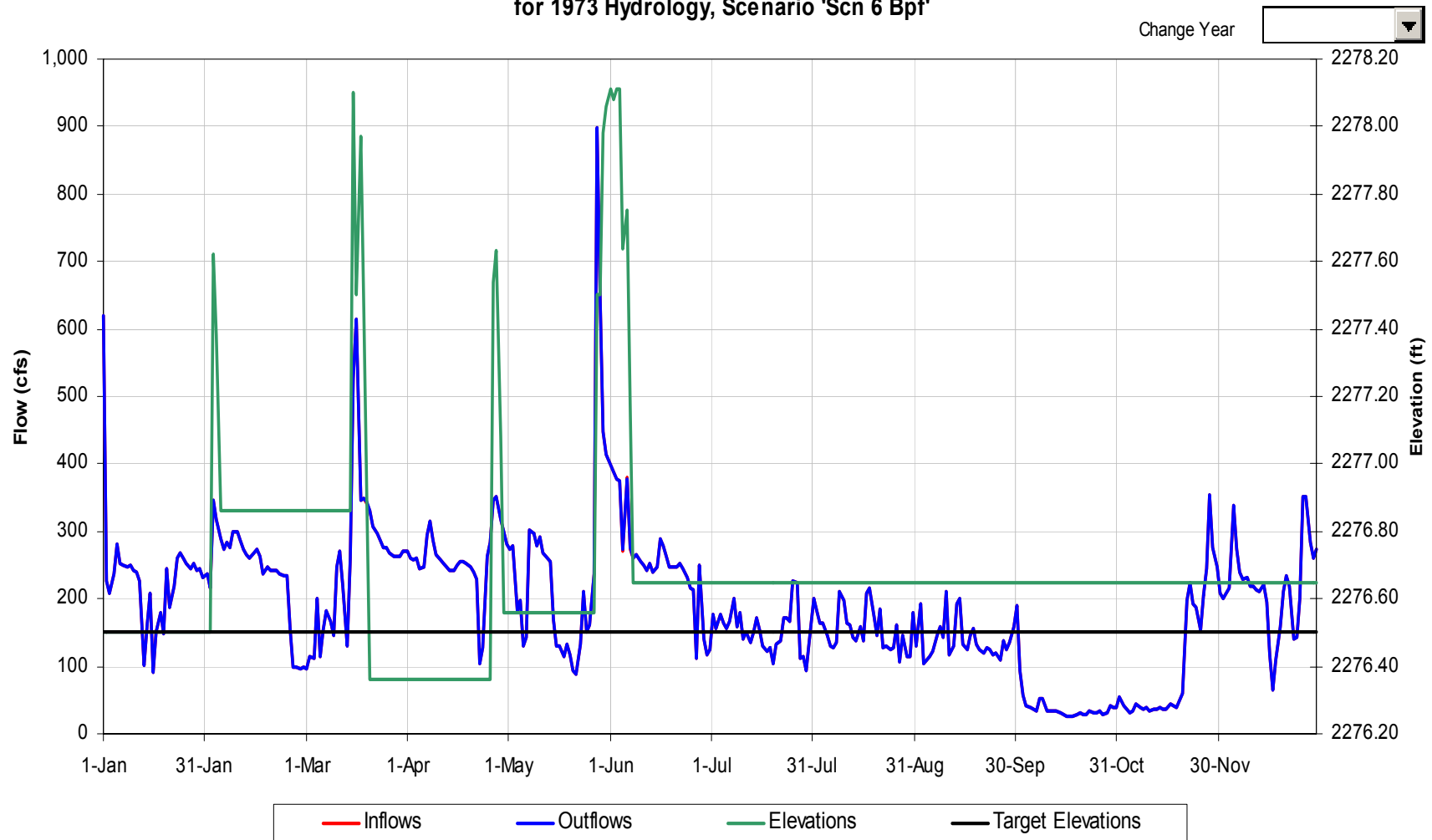
Tuckasegee Reservoir Operational Details for 1973 Hydrology, Scenario 'Scn 6 Bpf'
