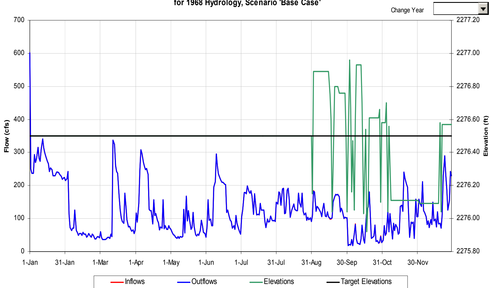
Tuckasegee Reservoir Operational Details for 1968 Hydrology, Scenario 'Base Case'
