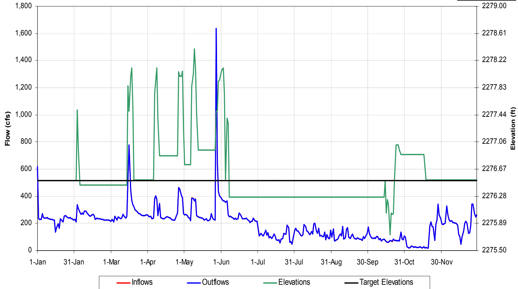
Tuckasegee Reservoir Operational Details for 1973 Hydrology, Scenario 'Scn 4 NcwrC Rc'
