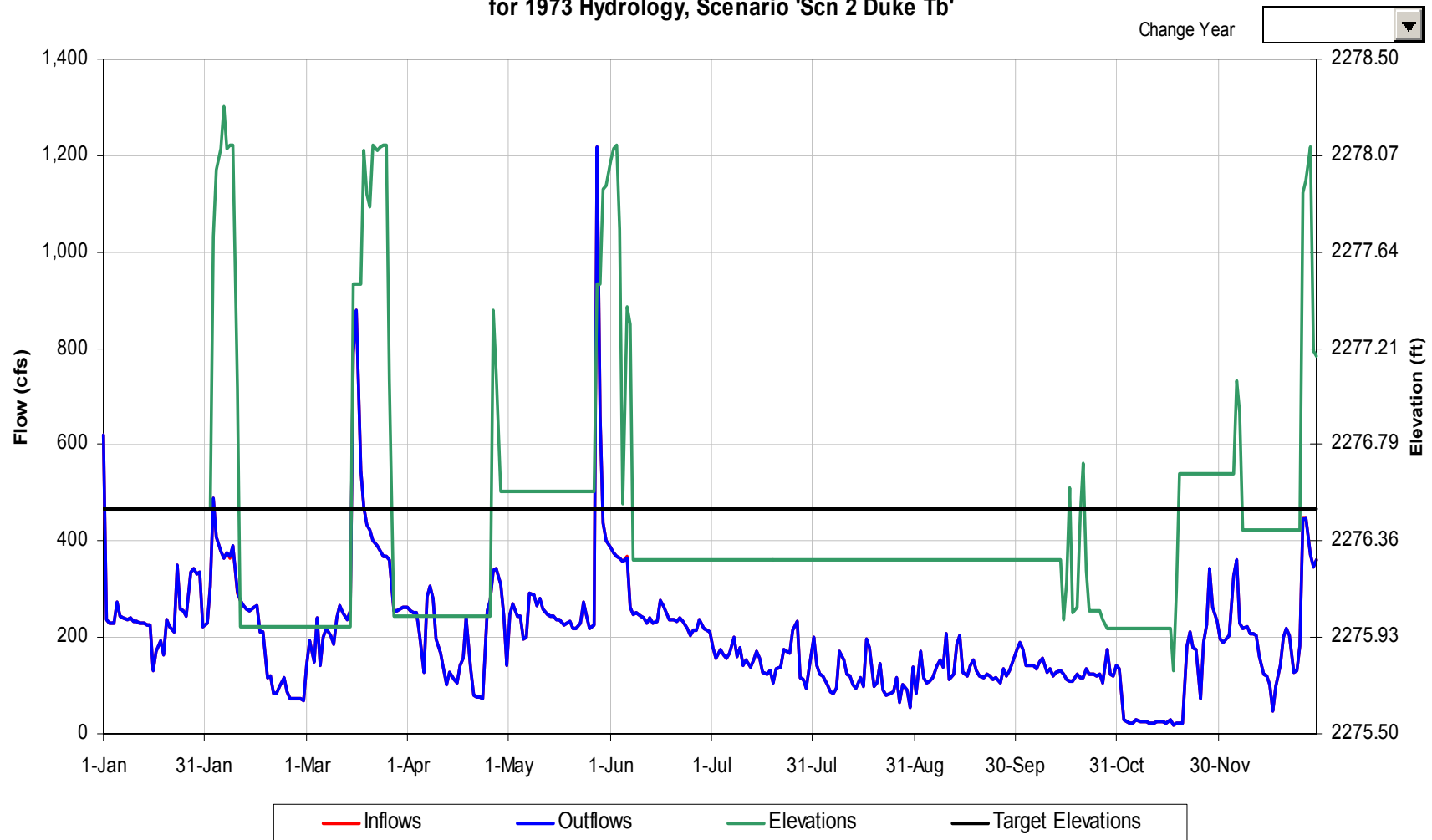
Tuckasegee Reservoir Operational Details for 1973 Hydrology, Scenario 'Scn 2 Duke Tb'
