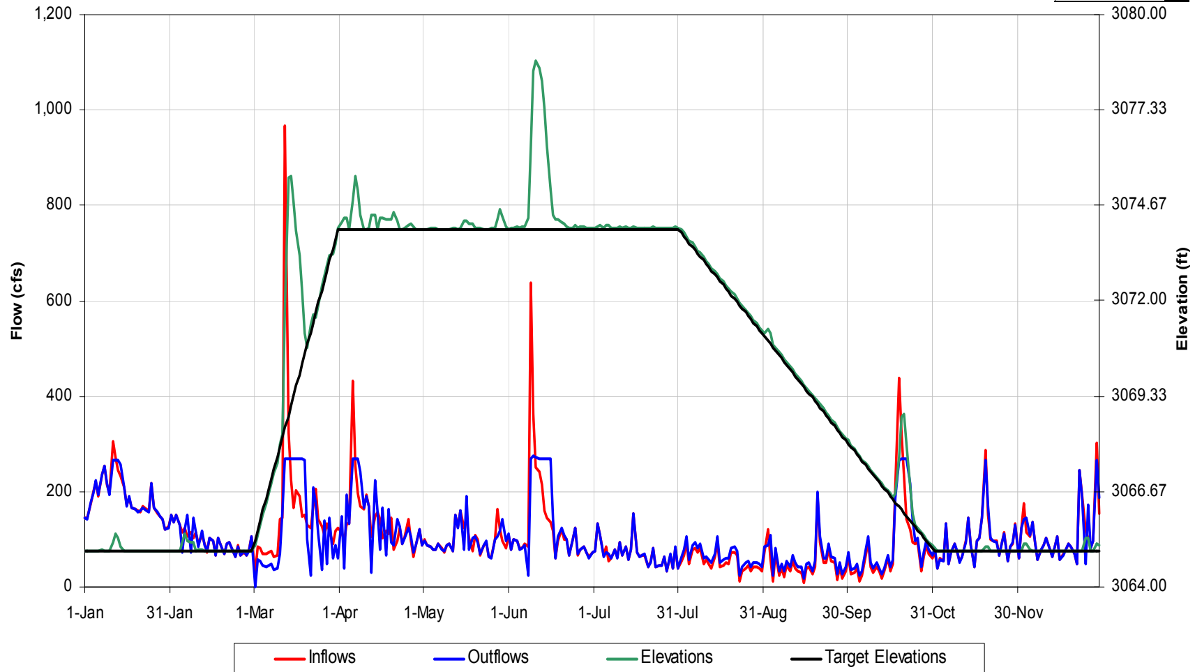
Tennessee Creek Reservoir Operational Details for 1968 Hydrology, Scenario 'Scn 4 Ncwr Rc'
