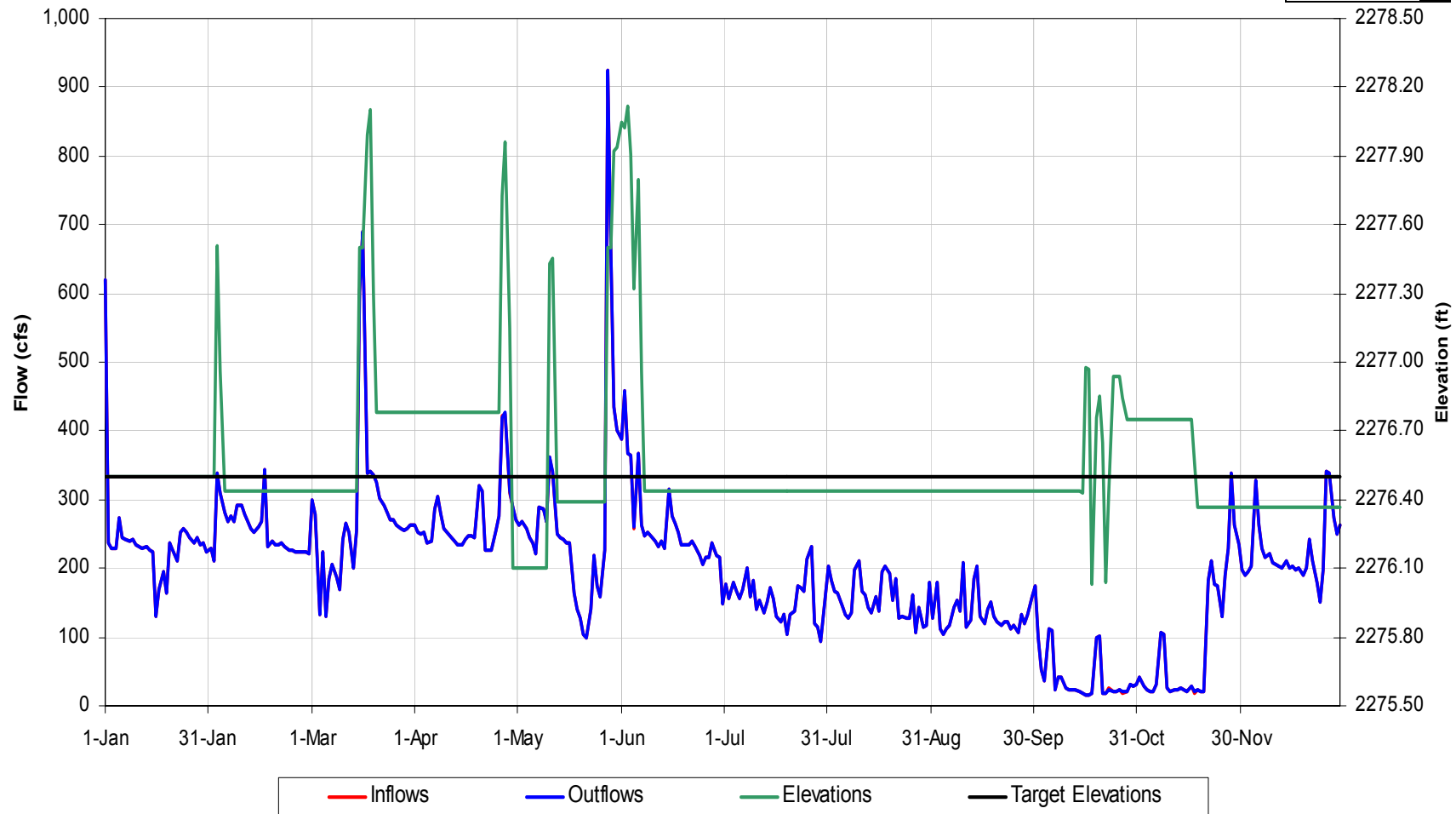
Tuckasegee Reservoir Operational Details for 1973 Hydrology, Scenario 'Scn 5 Rec Flows_'
