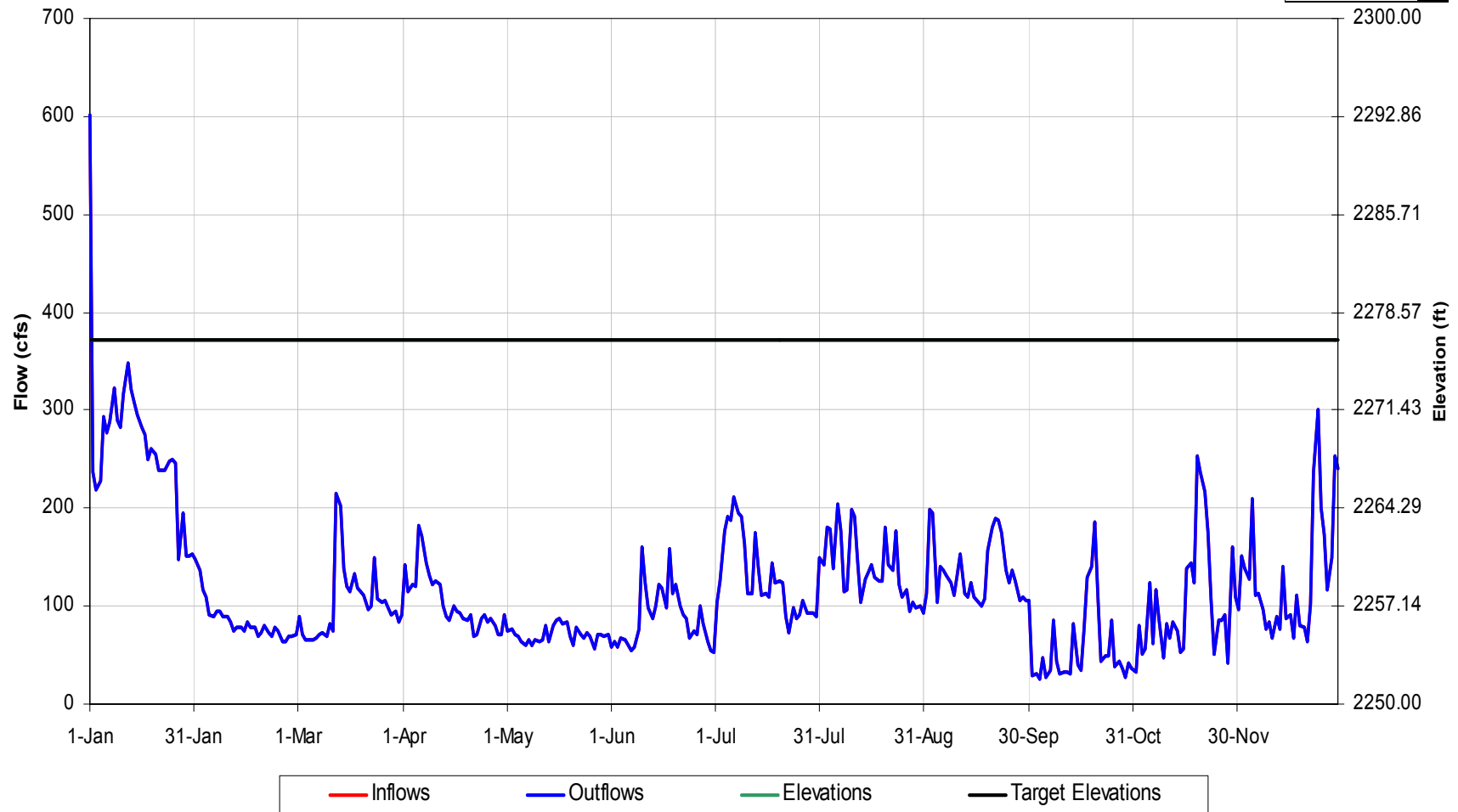
Tuckasegee Reservoir Operational Details for 1968 Hydrology, Scenario 'Scn 6 Bpf'
