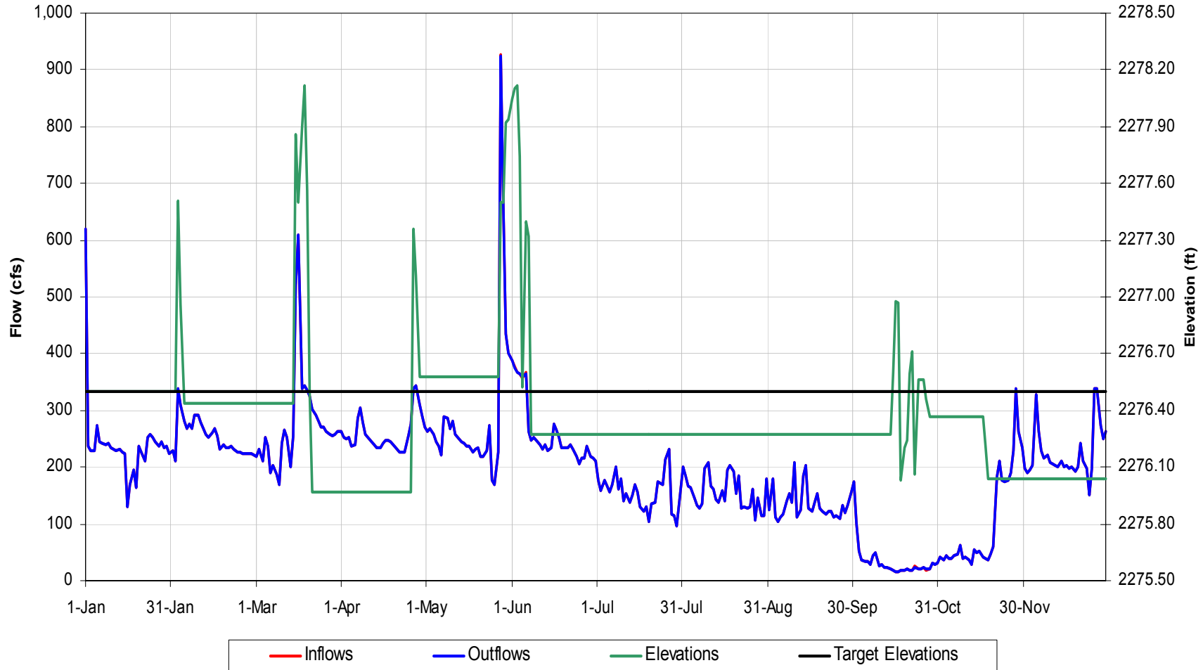
Tuckasegee Reservoir Operational Details for 1973 Hydrology, Scenario 'Base Case'
