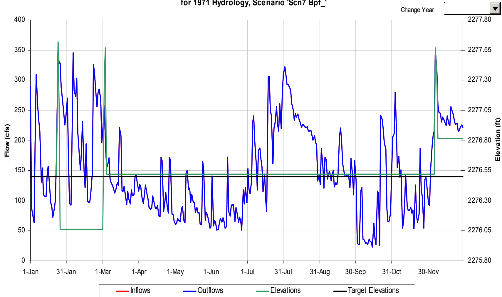
Tuckasegee Reservoir Operational Details for 1971 Hydrology, Scenario 'Scn7 Bpf_'
