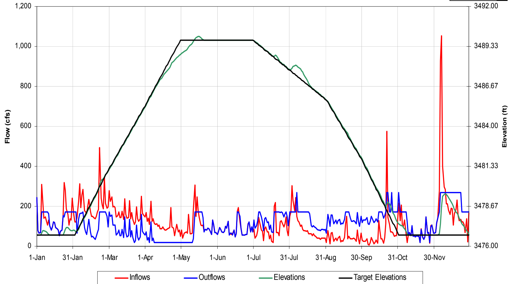
Thorpe Reservoir Operational Details for 1971 Hydrology, Scenario 'Scn 2 Duke Tb'
