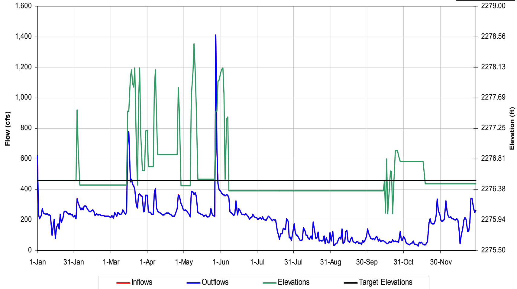
Tuckasegee Reservoir Operational Details for 1973 Hydrology, Scenario 'Scn 3 Lk Glvl Hoa Rc'
