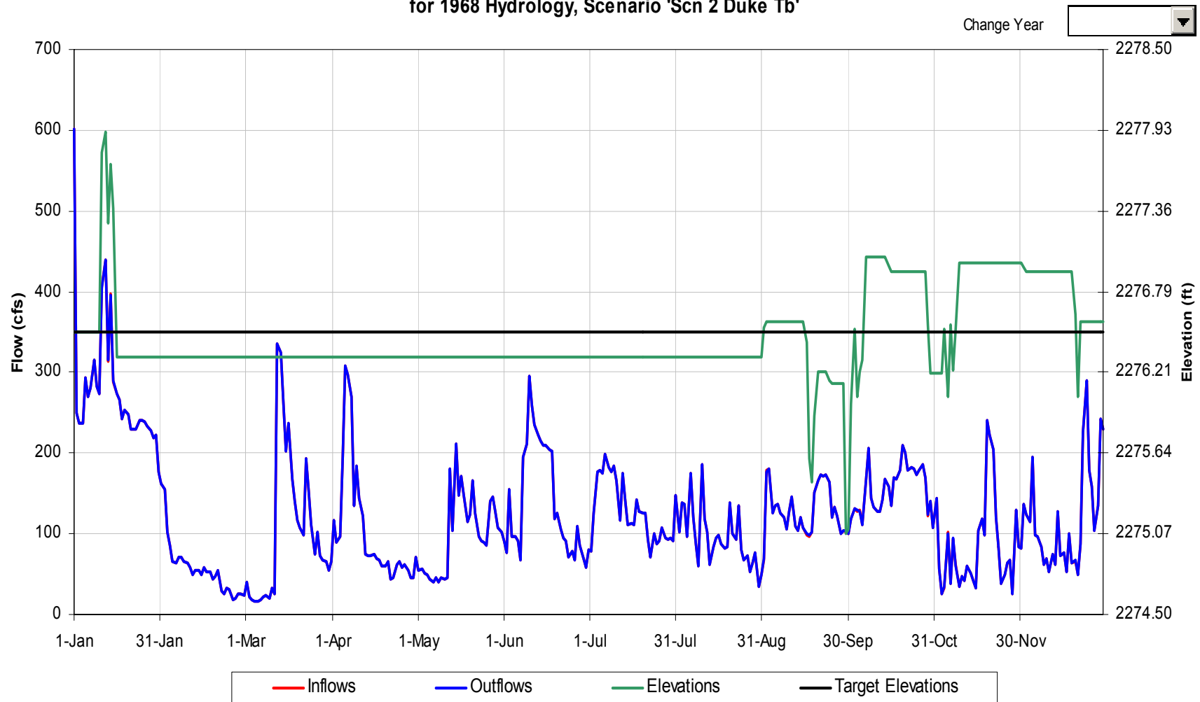
Tuckasegee Reservoir Operational Details for 1968 Hydrology, Scenario 'Scn 2 Duke Tb'
