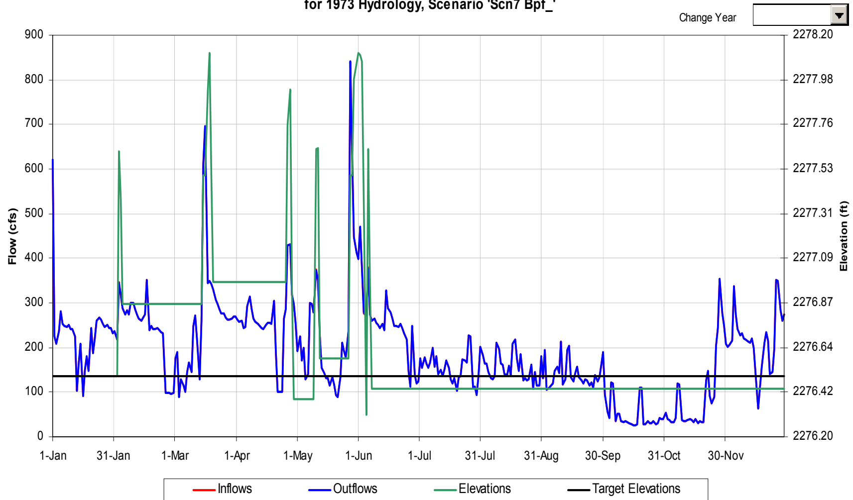
Tuckasegee Reservoir Operational Details for 1973 Hydrology, Scenario 'Scn7 Bpf_'
