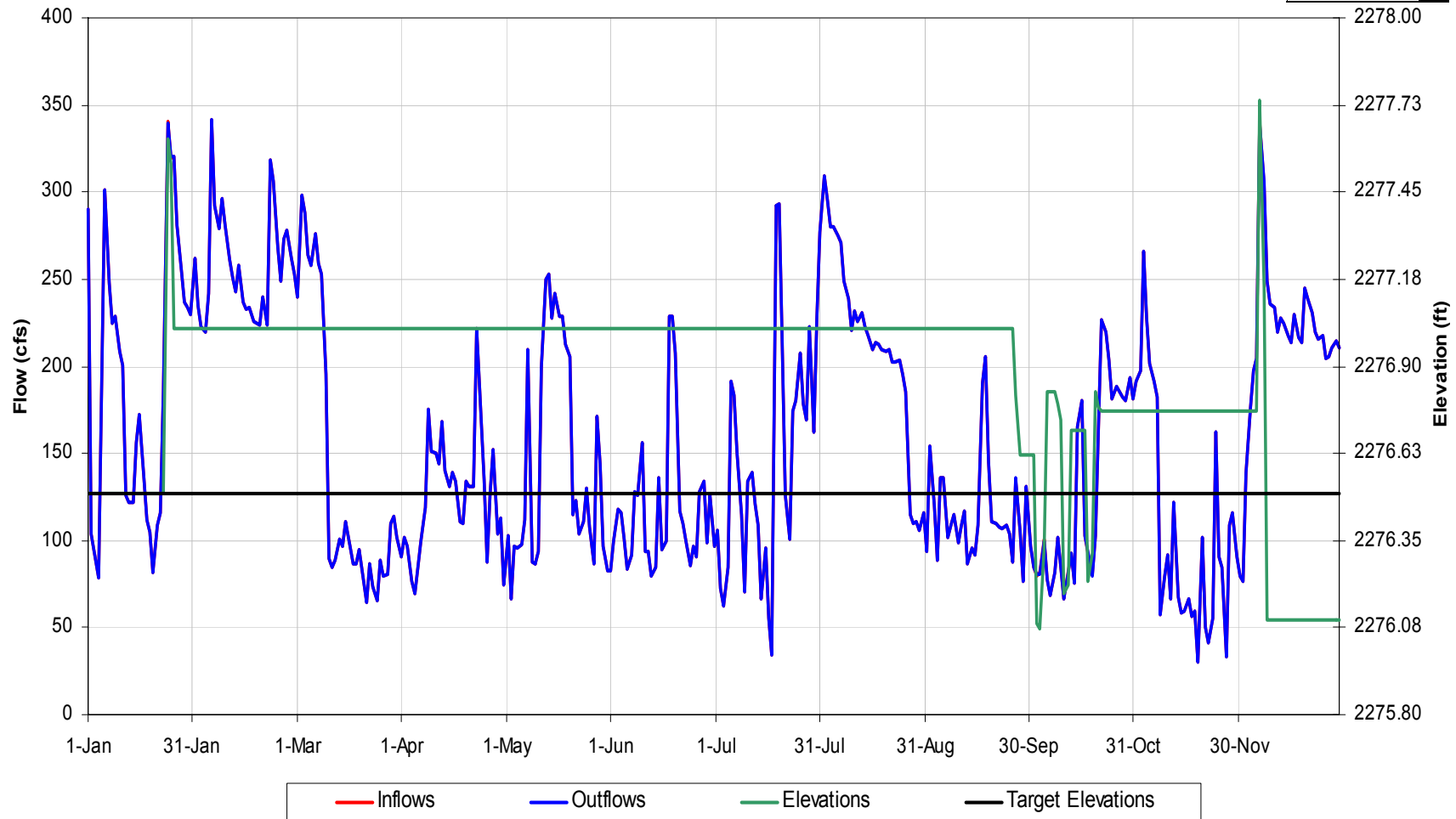
Tuckasegee Reservoir Operational Details for 1971 Hydrology, Scenario 'Scn 4 Ncwr Rc'
