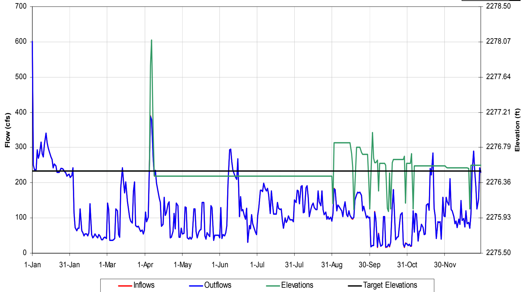
Tuckasegee Reservoir Operational Details for 1968 Hydrology, Scenario 'Scn 5a 2xrec Flows'
