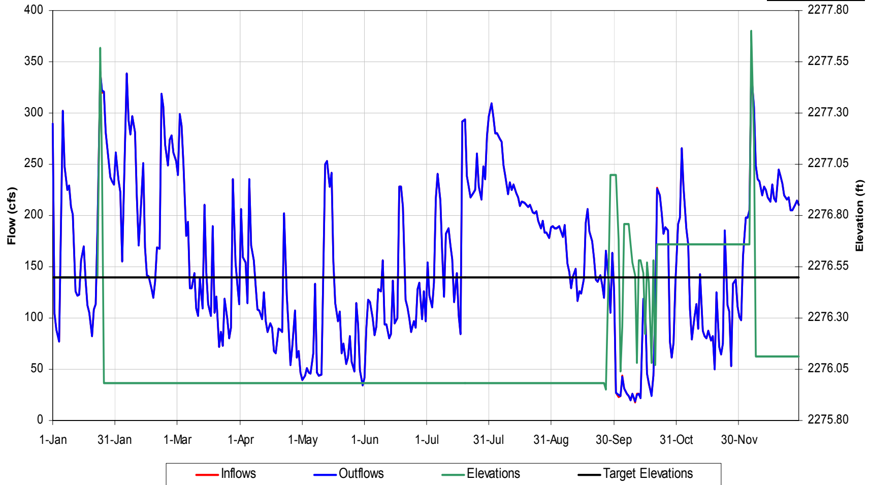
Tuckasegee Reservoir Operational Details for 1971 Hydrology, Scenario 'Base Case'
