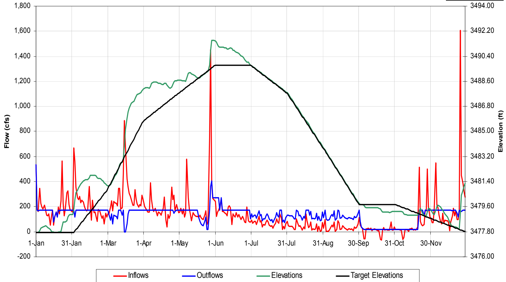
Thorpe Reservoir Operational Details for 1973 Hydrology, Scenario 'Scn 5 Rec Flows_'
