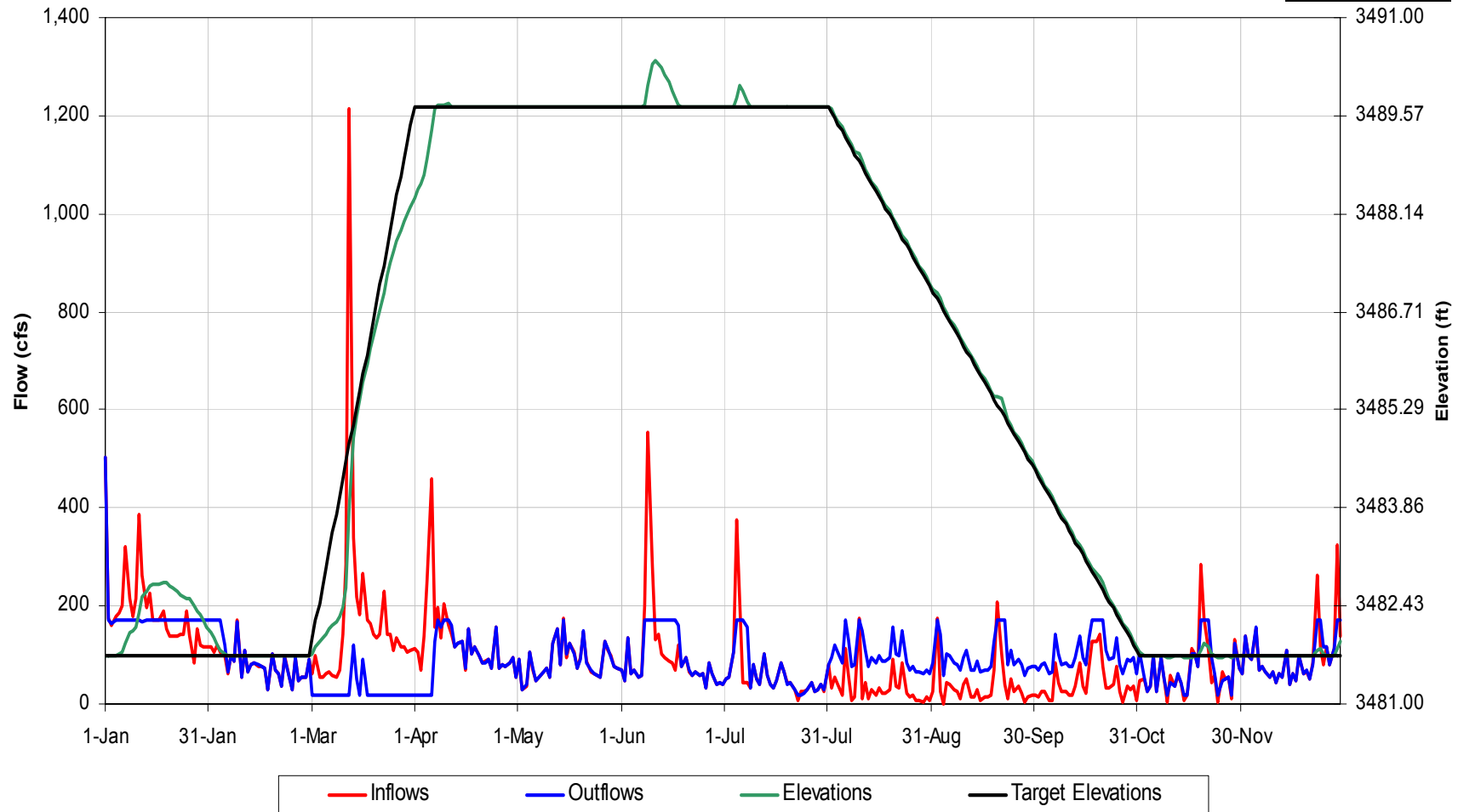
Thorpe Reservoir Operational Details for 1968 Hydrology, Scenario 'Scn 4 NcwrC Rc'
