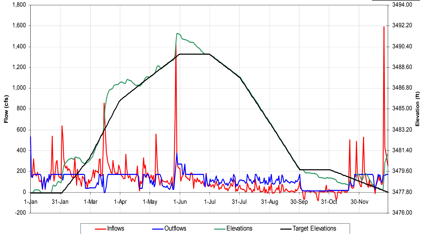
Thorpe Reservoir Operational Details for 1973 Hydrology, Scenario 'Scn7 Bpf_'
