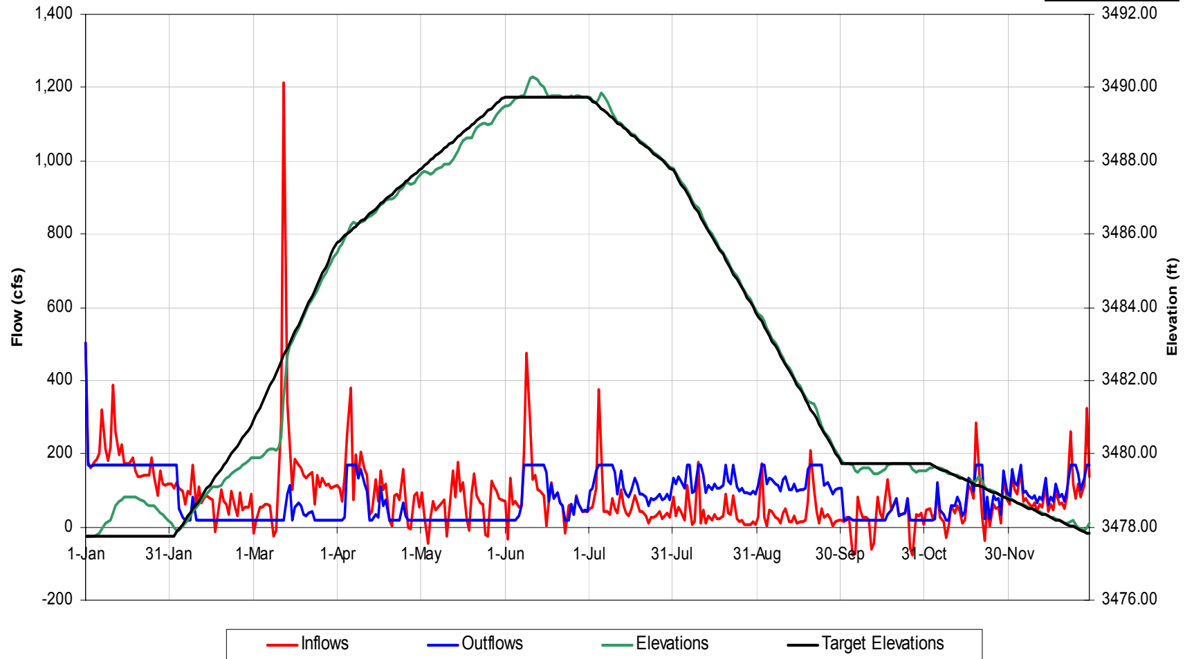
Thorpe Reservoir Operational Details for 1968 Hydrology, Scenario 'Scn 5a 2xrec Flows'
