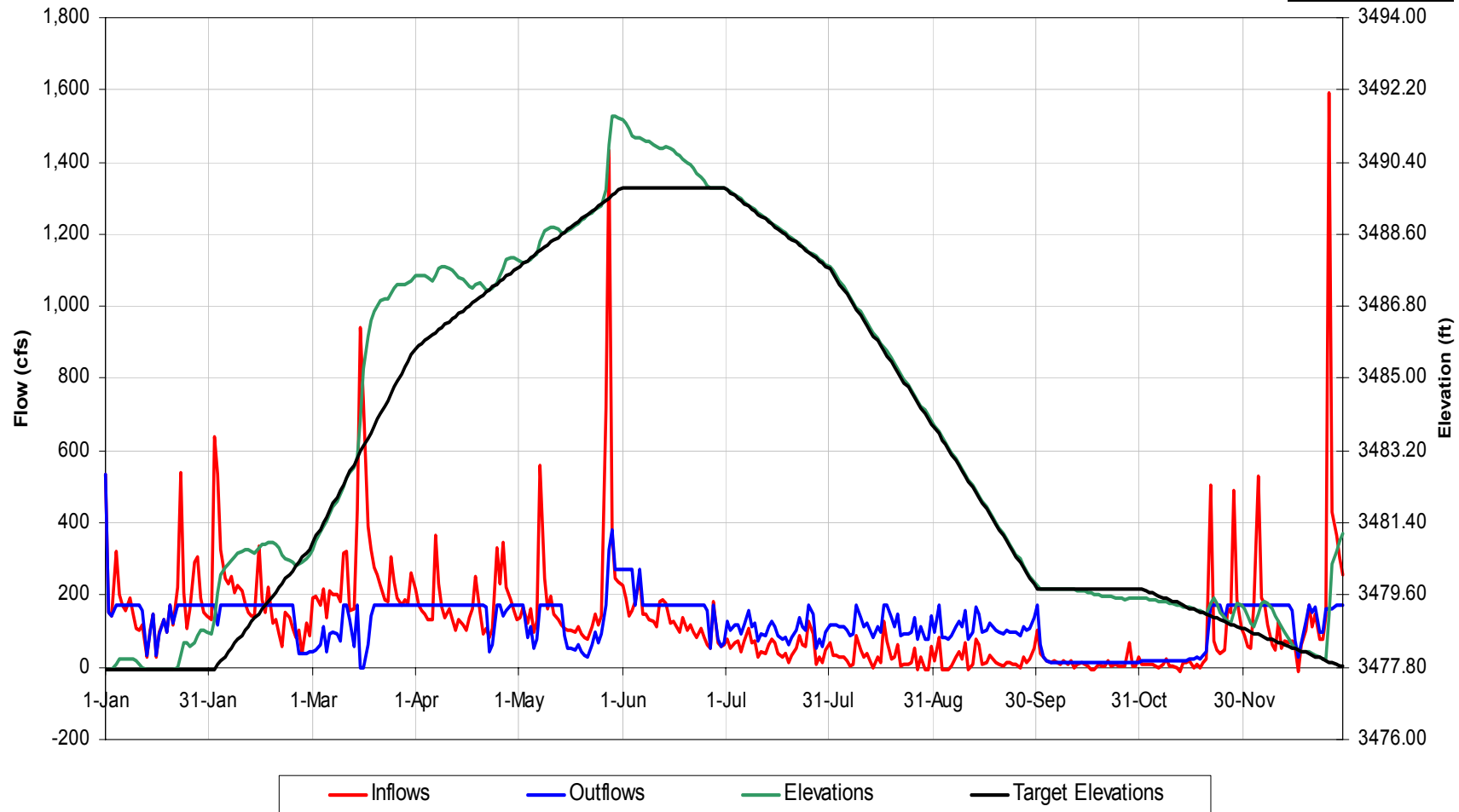
Thorpe Reservoir Operational Details for 1973 Hydrology, Scenario 'Scn 6 Bpf'
