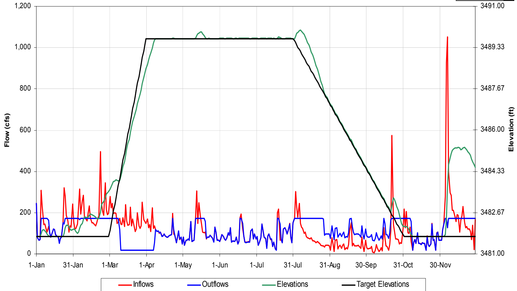
Thorpe Reservoir Operational Details for 1971 Hydrology, Scenario 'Scn 4 NcwrC'
