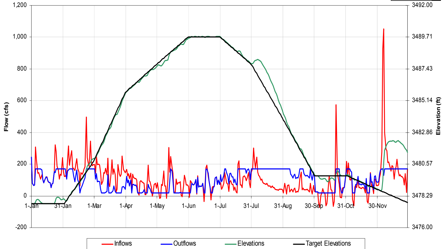
Thorpe Reservoir Operational Details for 1971 Hydrology, Scenario 'Scn 5a 2xrec Flows'
