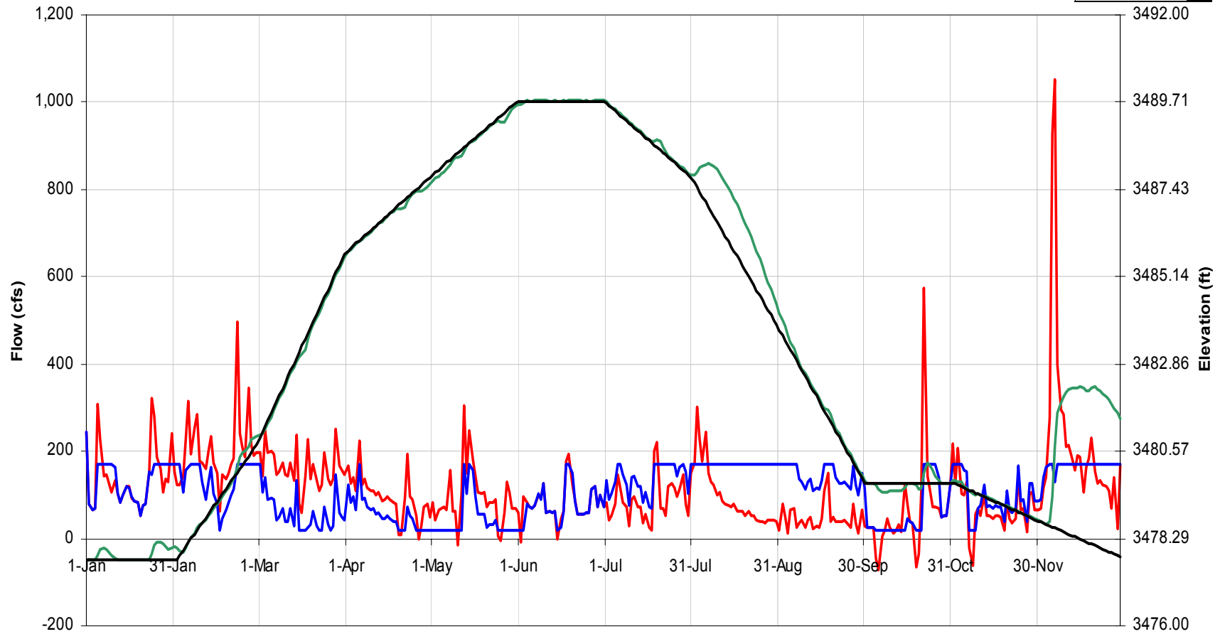
Thorpe Reservoir Operational Details for 1971 Hydrology, Scenario 'Scn 5 Rec Flows_'
