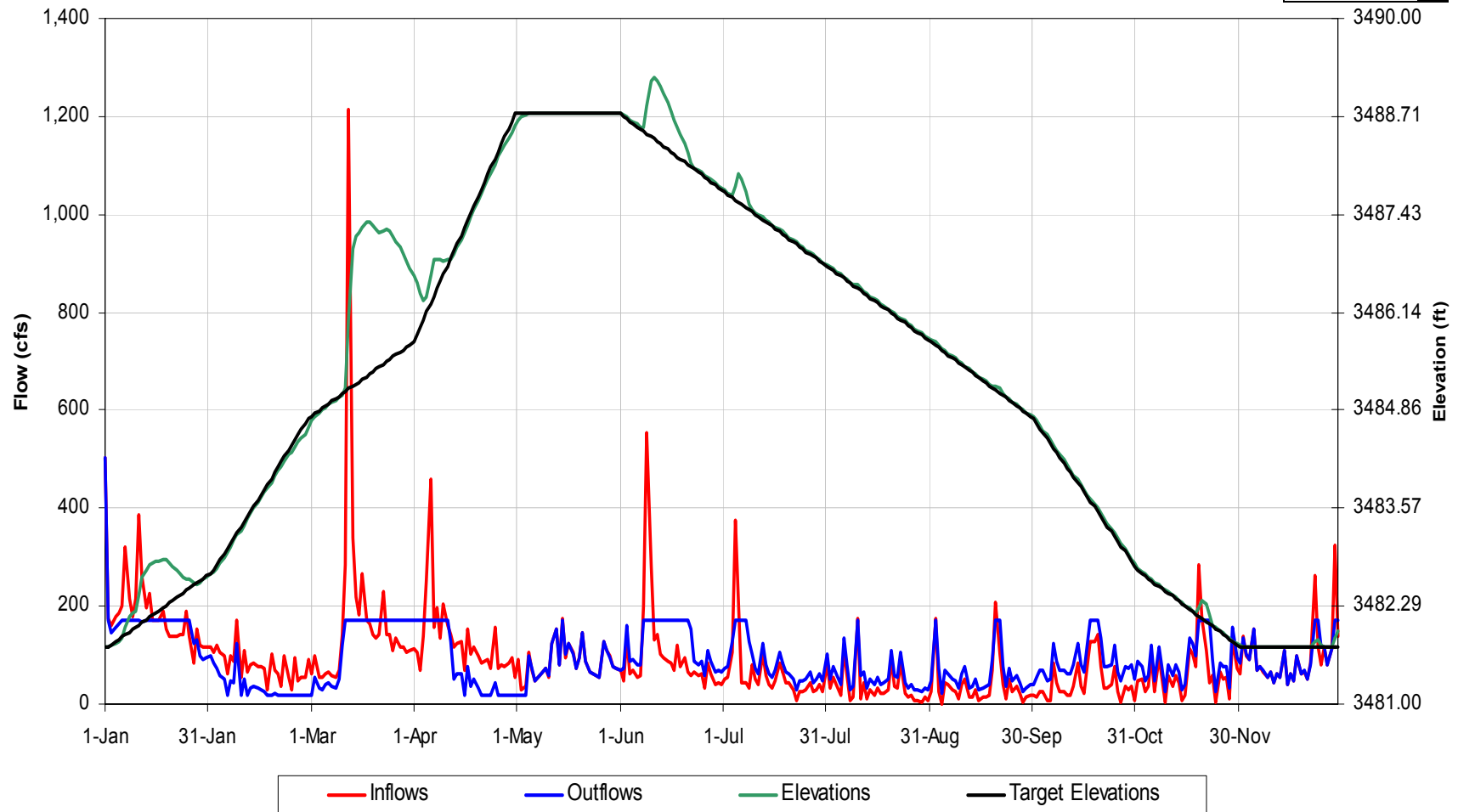
Thorpe Reservoir Operational Details for 1968 Hydrology, Scenario 'Scn 3 Lk Glvl Hoa Rc'
