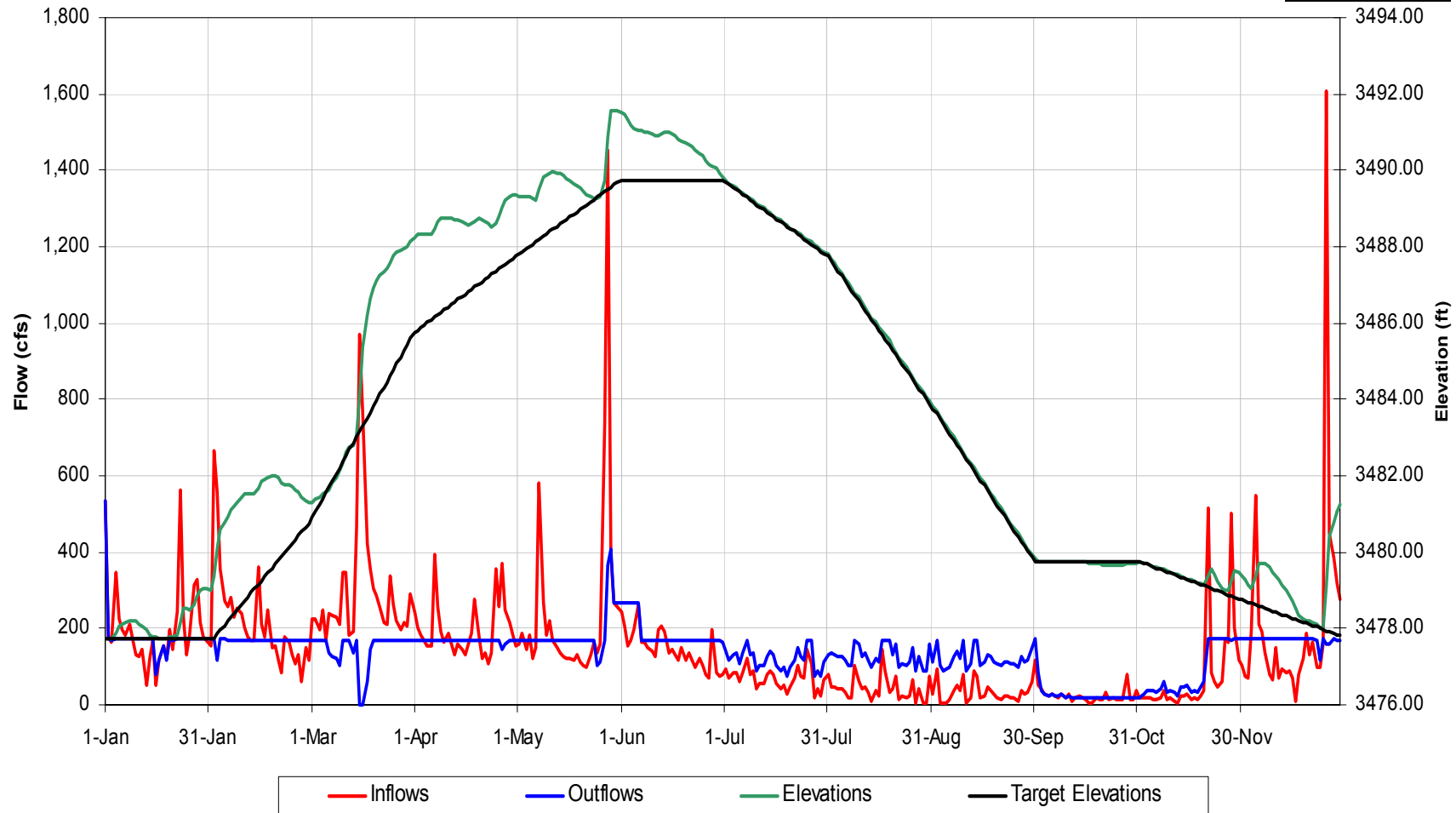
Thorpe Reservoir Operational Details for 1973 Hydrology, Scenario 'Base Case'
