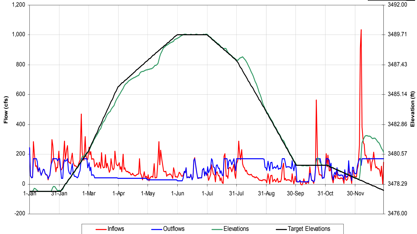
Thorpe Reservoir Operational Details for 1971 Hydrology, Scenario 'Scn 6 Bpf'
