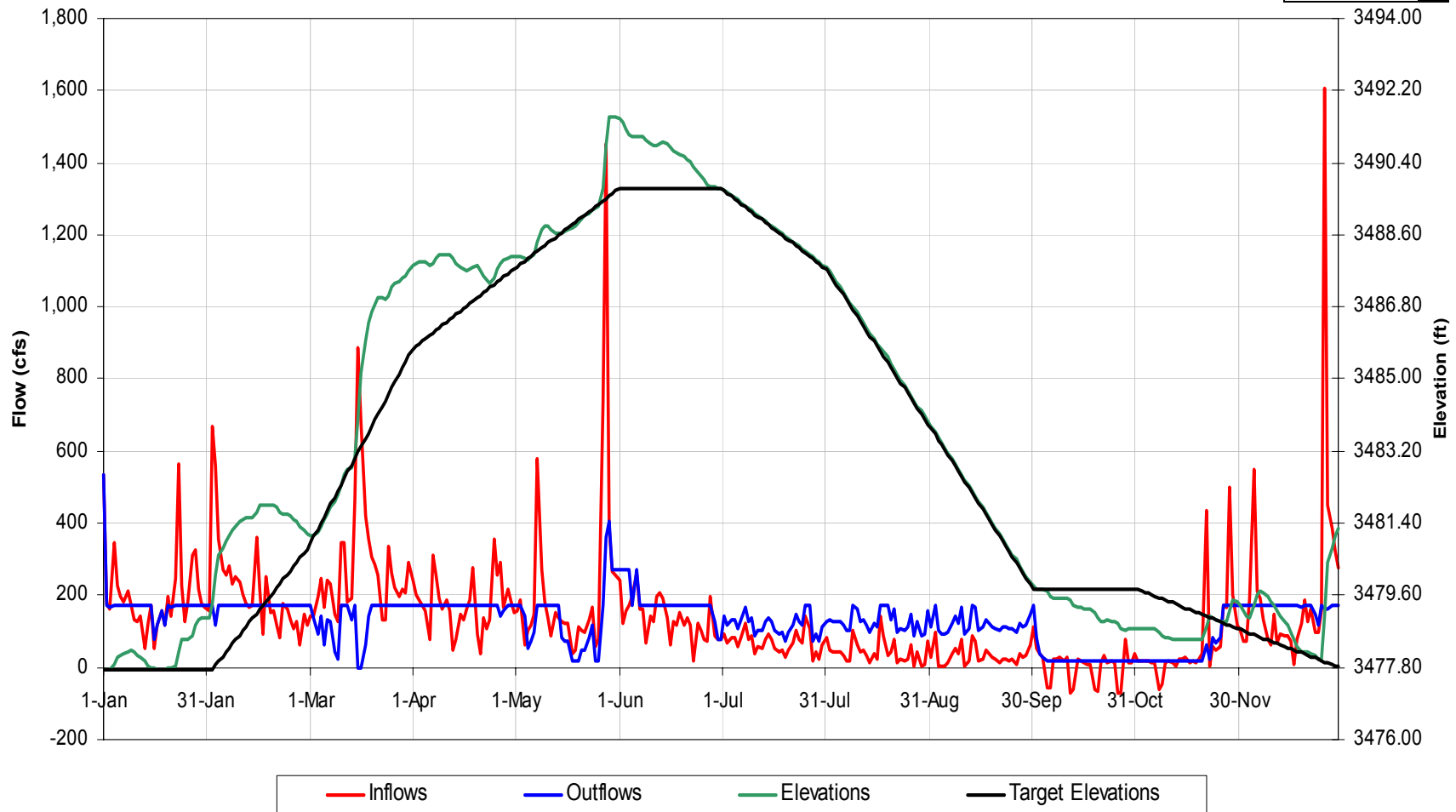
Thorpe Reservoir Operational Details for 1973 Hydrology, Scenario 'Scn 5a 2xrec Flows'
