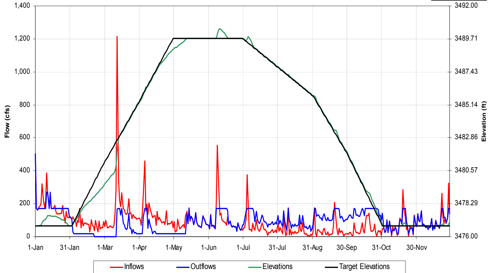
Thorpe Reservoir Operational Details for 1968 Hydrology, Scenario 'Scn 2 Duke Tb'
