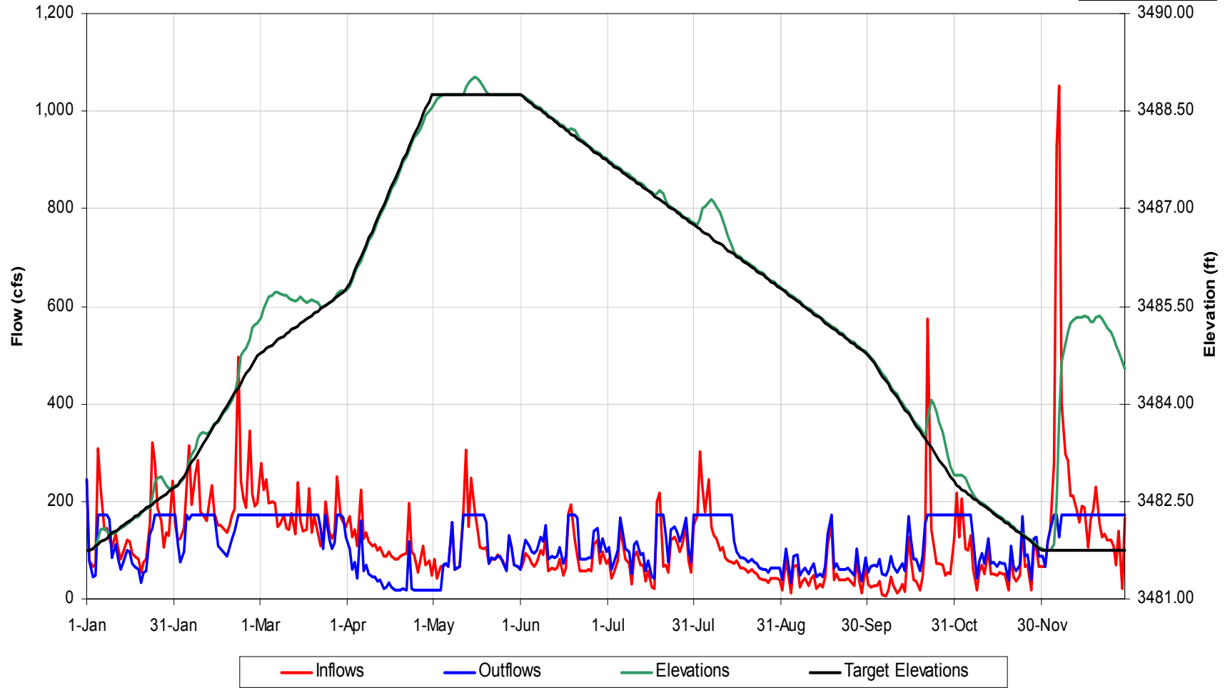
Thorpe Reservoir Operational Details for 1971 Hydrology, Scenario 'Scn 3 Lk Glvl Hoa Rc'
