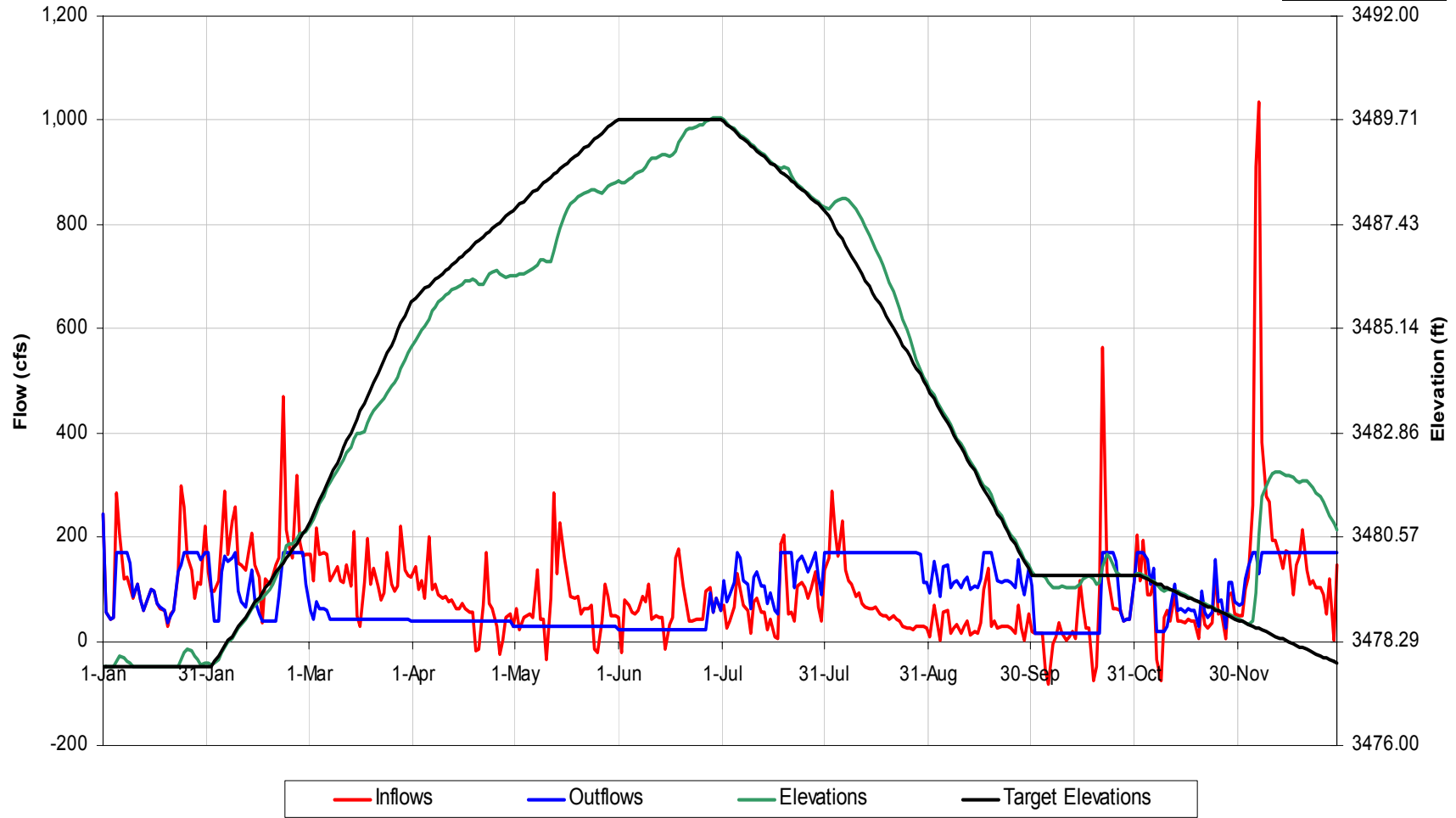
Thorpe Reservoir Operational Details for 1971 Hydrology, Scenario 'Scn7 Bpf_'
