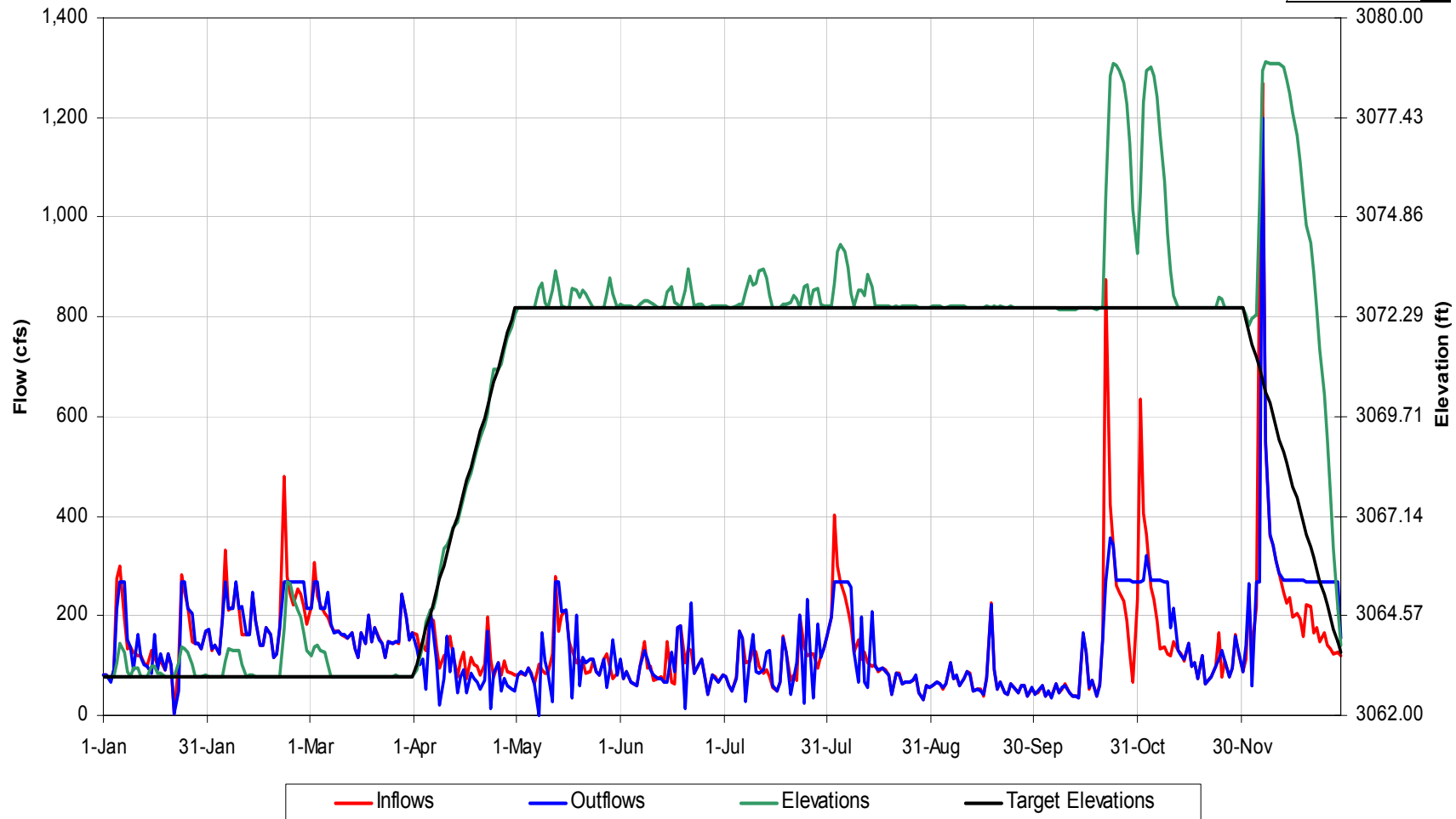
Tennessee Creek Reservoir Operational Details for 1971 Hydrology, Scenario 'Scn 5 Rec Flows_'
