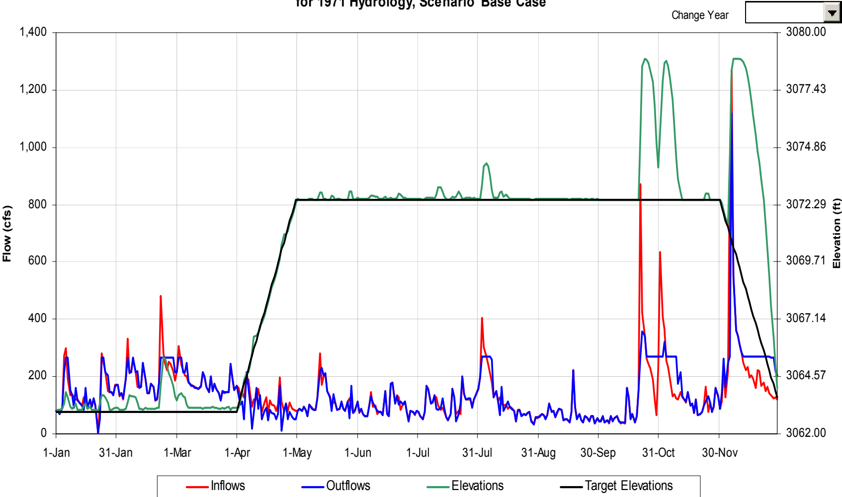
Tennessee Creek Reservoir Operational Details for 1971 Hydrology, Scenario 'Base Case'
