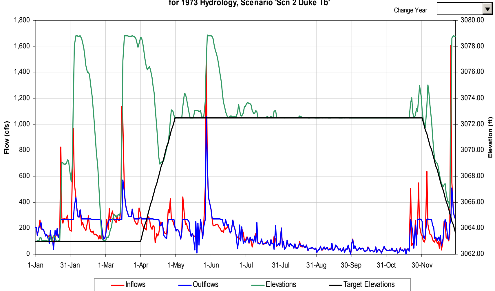
Tennessee Creek Reservoir Operational Details for 1973 Hydrology, Scenario 'Scn 2 Duke Tb'
