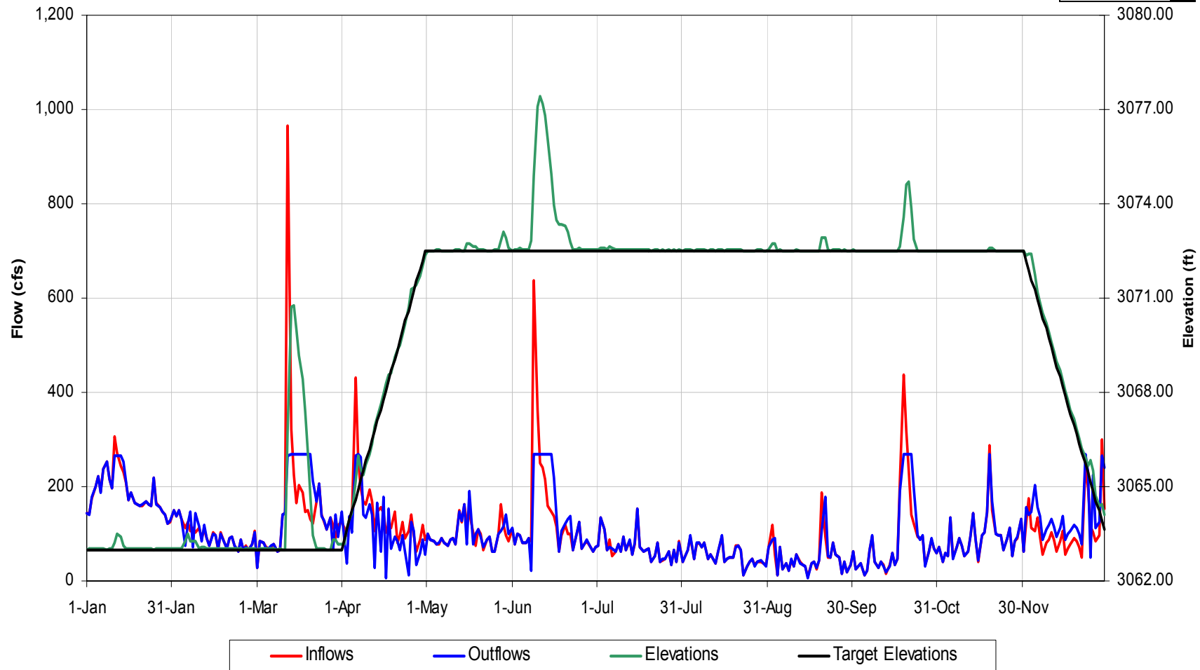
Tennessee Creek Reservoir Operational Details for 1968 Hydrology, Scenario 'Scn 2 Duke Tb'
