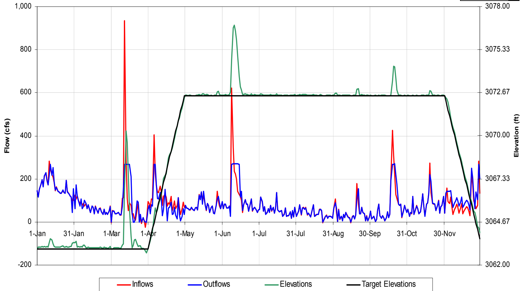
Tennessee Creek Reservoir Operational Details for 1968 Hydrology, Scenario 'Scn7 Bpf_'
