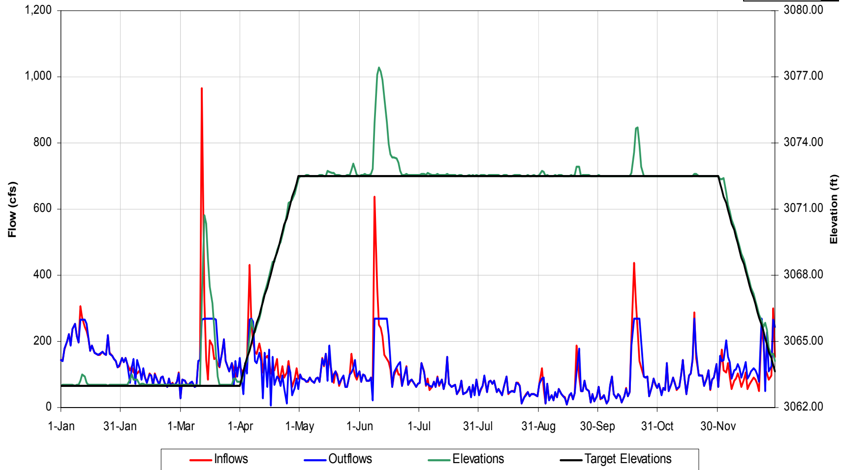
Tennessee Creek Reservoir Operational Details for 1968 Hydrology, Scenario 'Scn 5a 2xrec Flows'
