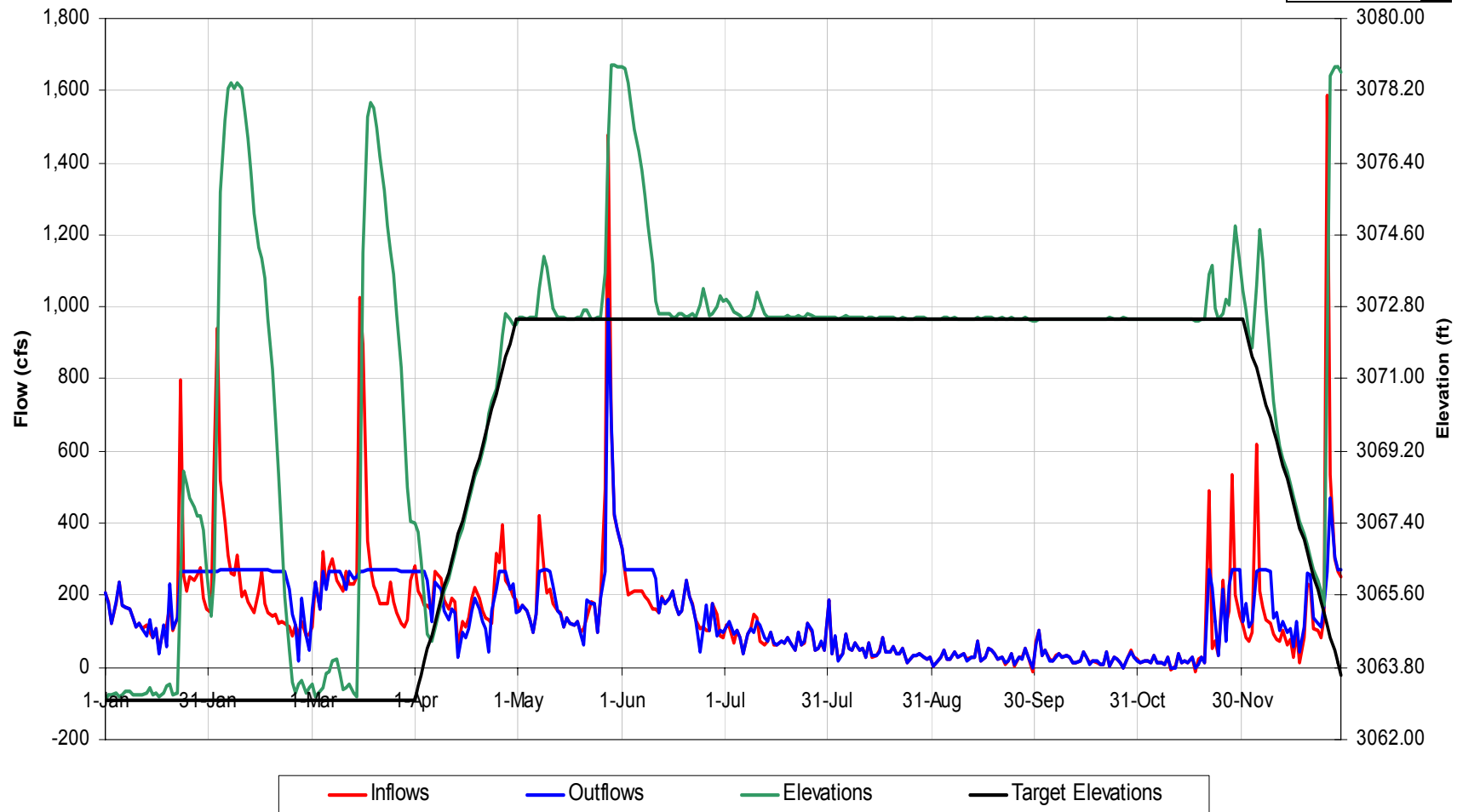
Tennessee Creek Reservoir Operational Details for 1973 Hydrology, Scenario 'Scn7 Bpf_'
