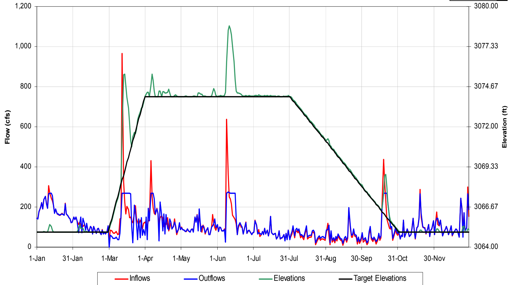
Tennessee Creek Reservoir Operational Details for 1968 Hydrology, Scenario 'Scn 4 NcwrC Rc'
