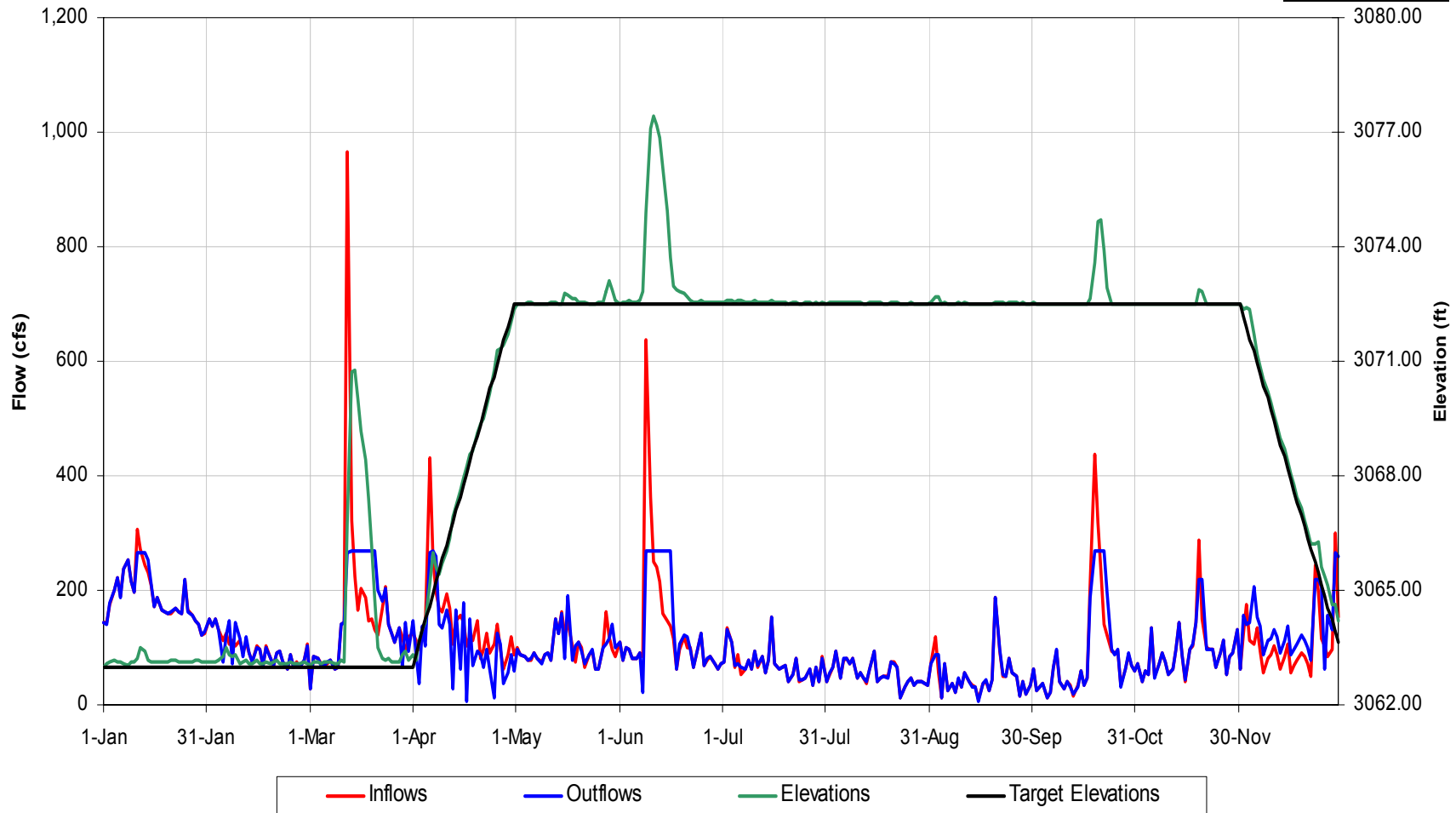
Tennessee Creek Reservoir Operational Details for 1968 Hydrology, Scenario 'Scn 3 Lk Glvl Hoa Rc'
