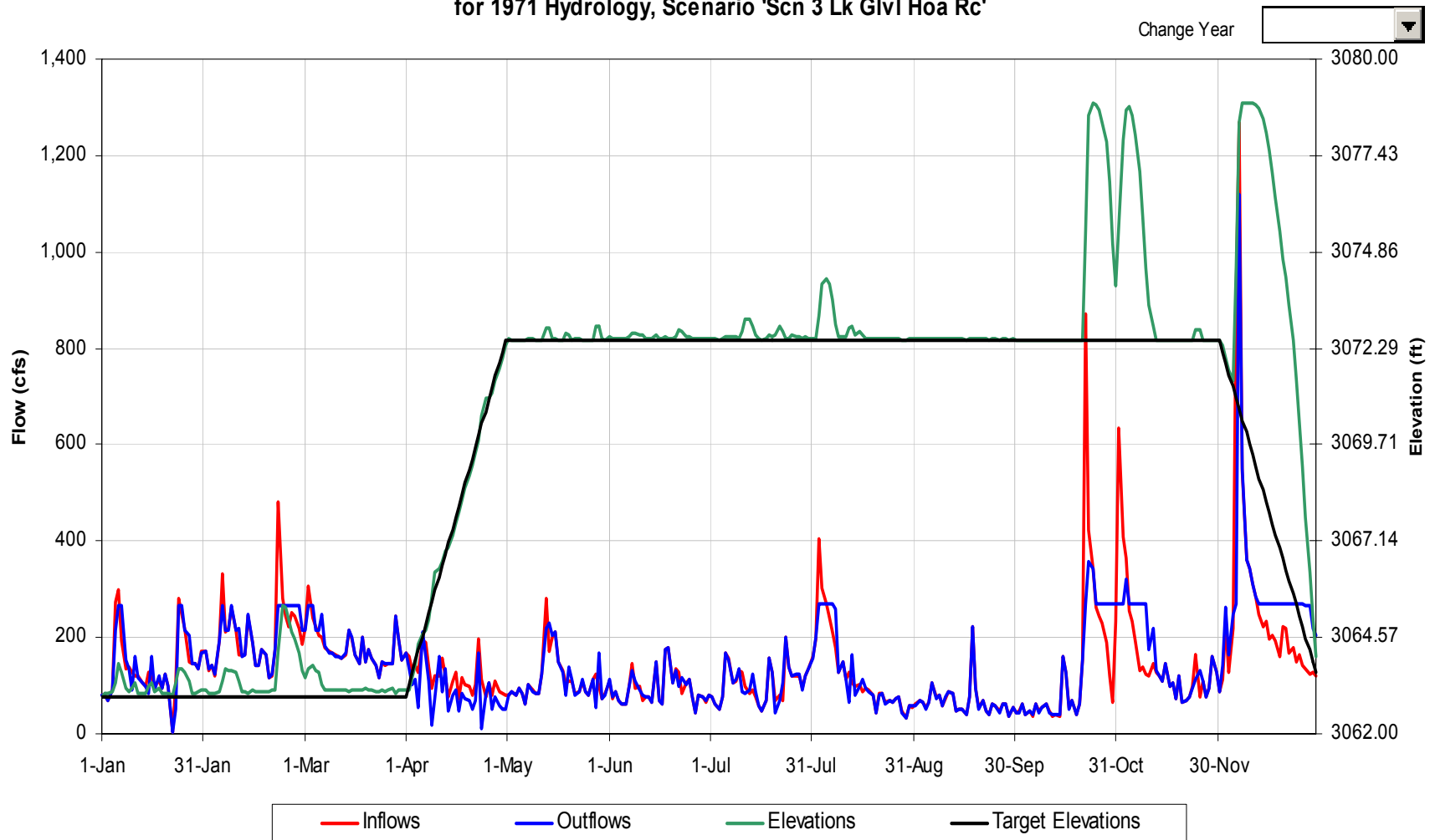
Tennessee Creek Reservoir Operational Details for 1971 Hydrology, Scenario 'Scn 3 Lk Glvl Hoa Rc'
