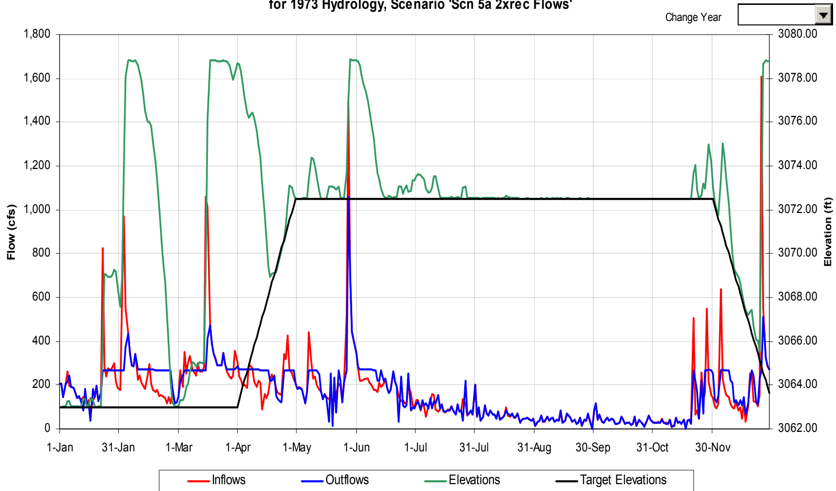
Tennessee Creek Reservoir Operational Details for 1973 Hydrology, Scenario 'Scn 5a 2xrec Flows'
