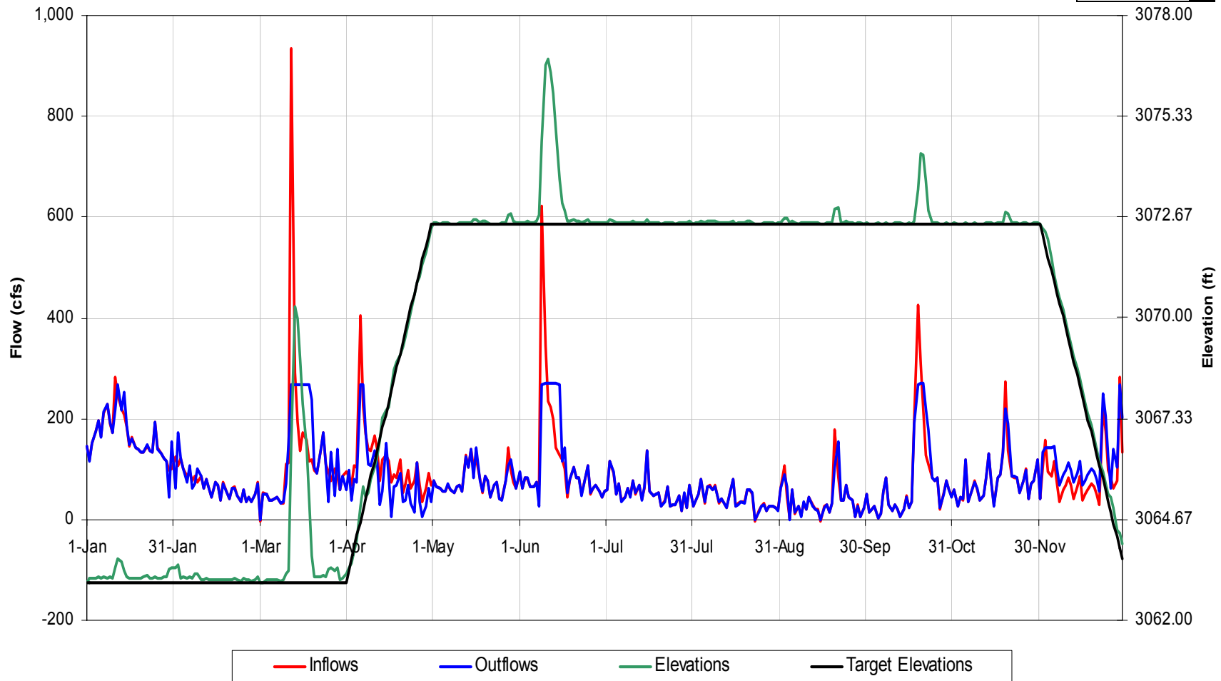
Tennessee Creek Reservoir Operational Details for 1968 Hydrology, Scenario 'Scn 6 Bpf'
