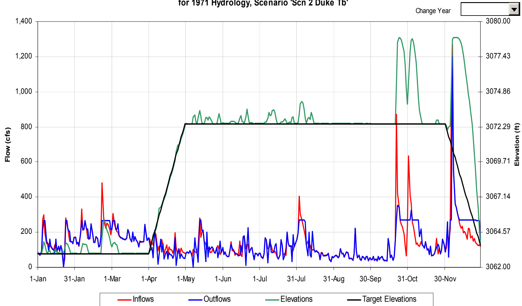
Tennessee Creek Reservoir Operational Details for 1971 Hydrology, Scenario 'Scn 2 Duke Tb'
