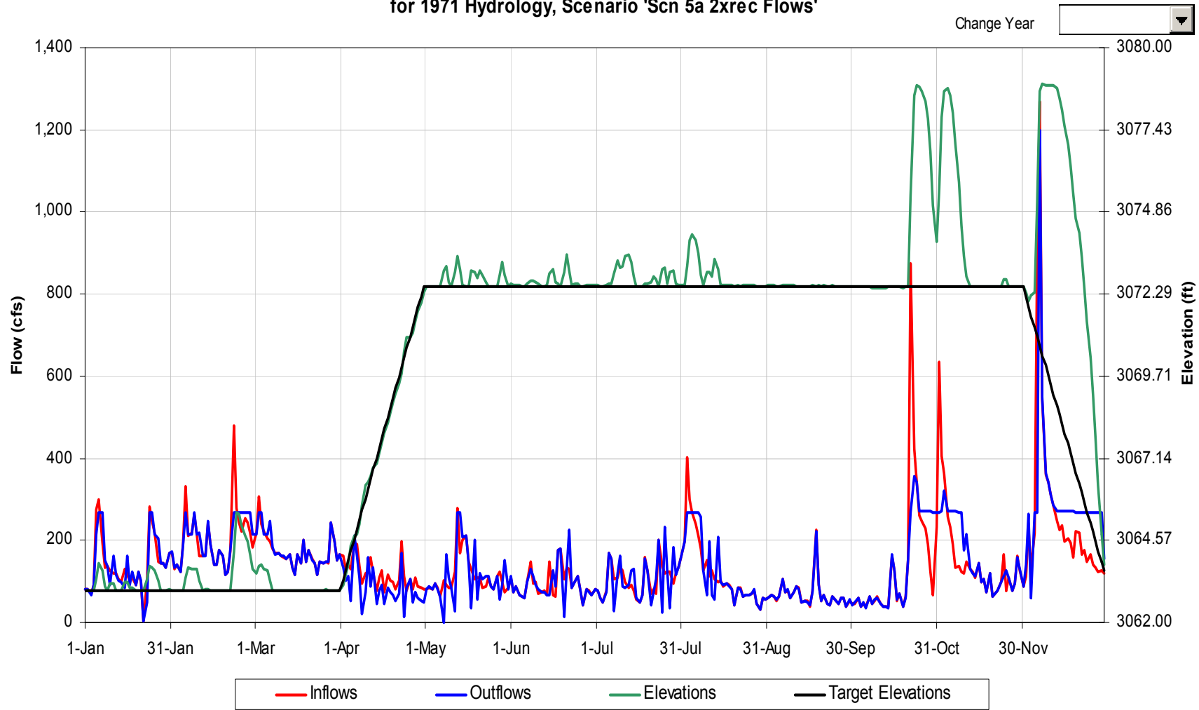
Tennessee Creek Reservoir Operational Details for 1971 Hydrology, Scenario 'Scn 5a 2xrec Flows'
